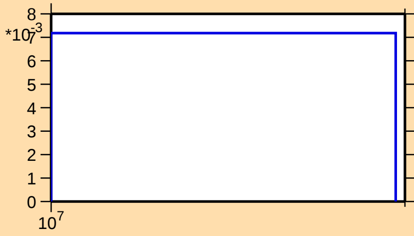
\sigma vs. E for ^{124}\text{Sn}(n,3n)
