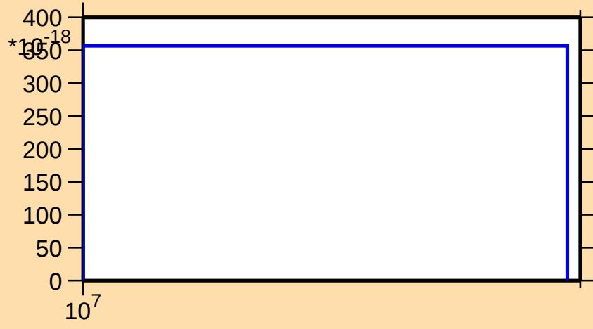
\sigma vs. E for ^{124}\text{Sn}(n,\text{nd})
