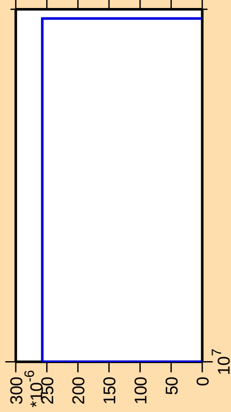
\Delta\sigma/\sigma vs. E for ^{124}\text{Sn}(n,\text{nt})
