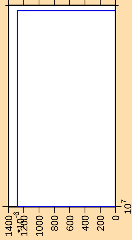
\Delta\sigma/\sigma vs. E for ^{124}\text{Sn}(n,\text{nd})
