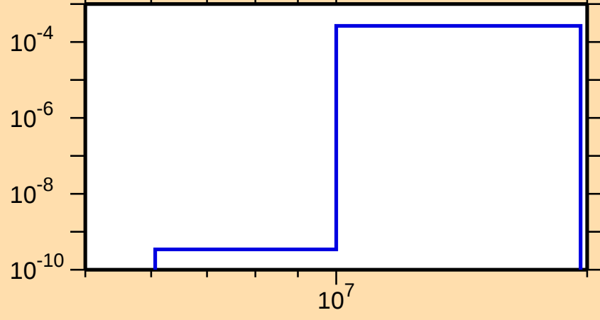
\sigma vs. E for ^{124}\text{Sn}(n,p)
