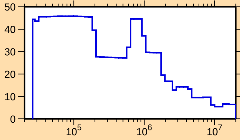
\Delta\sigma/\sigma vs. E for ^{125}\text{Sn}(n,\text{nonel.})
