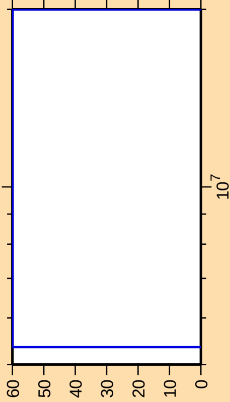
\Delta\sigma/\sigma vs. E for ^{125}\text{Sn}(n,n_1)
