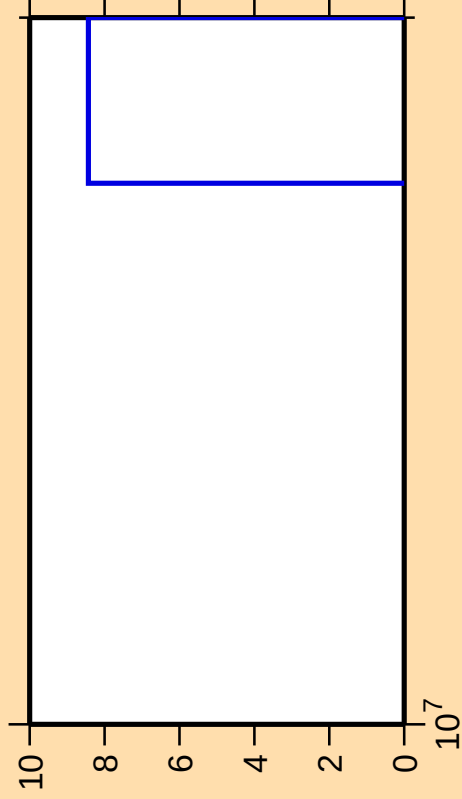
\Delta\sigma/\sigma vs. E for ^{125}\text{Sn}(n,2np)
