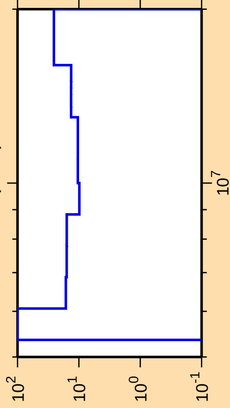
\Delta\sigma/\sigma vs. E for ^{125}\text{Sn}(n,2n)
