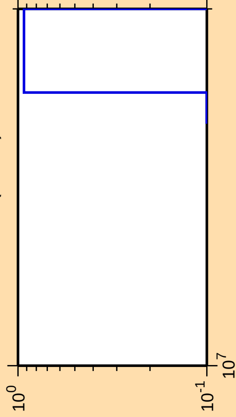
\Delta\sigma/\sigma vs. E for ^{125}\text{Sn}(n,2n\alpha)
