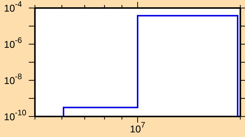
\sigma vs. E for ^{125}\text{Sn}(n,\alpha)
