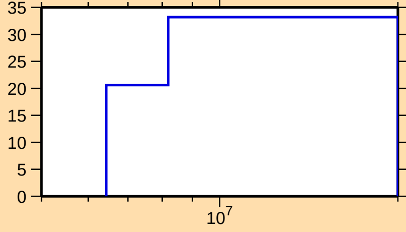
\Delta\sigma/\sigma vs. E for ^{125}\text{Sn}(n,\text{ncont.})
