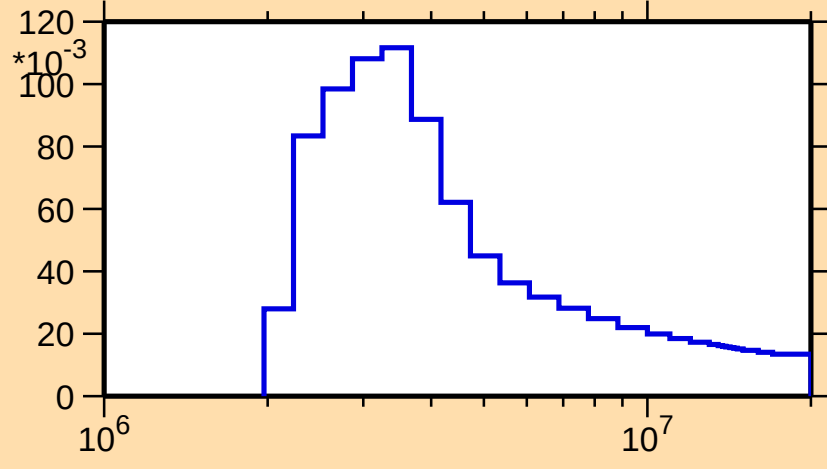
\sigma vs. E for ^{126}\text{Sn}(n,n_2)
