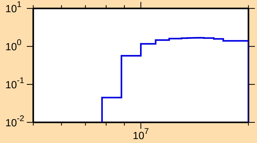
\sigma vs. E for ^{126}\text{Sn}(n,2n)
