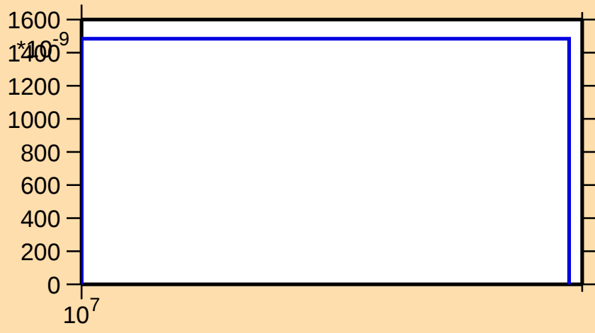
\sigma vs. E for ^{126}\text{Sn}(n,d)
