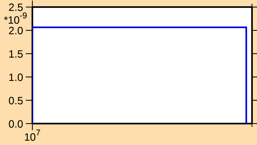
\sigma vs. E for ^{126}\text{Sn}(n,n\alpha)
