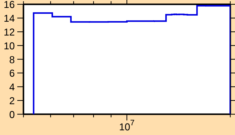
\Delta\sigma/\sigma vs. E for ^{127}\text{Sn}(n,\text{nonel.})
