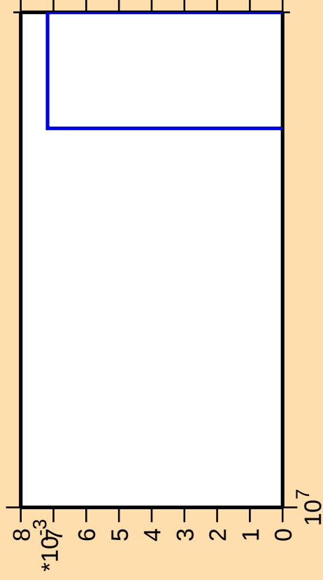
\Delta\sigma/\sigma vs. E for ^{127}\text{Sn}(n,2np)
