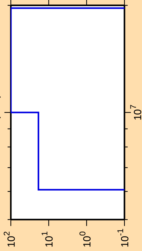
\Delta\sigma/\sigma vs. E for ^{127}\text{Sn}(n,\alpha)
