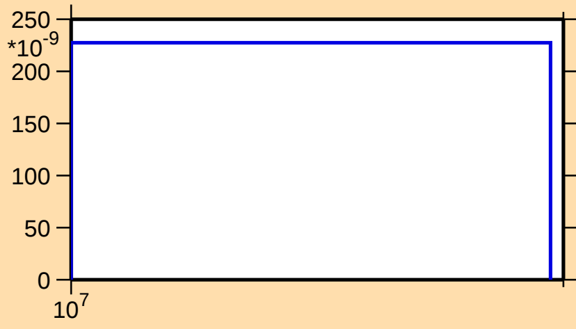
\sigma vs. E for ^{127}\text{Sn}(n,t)
