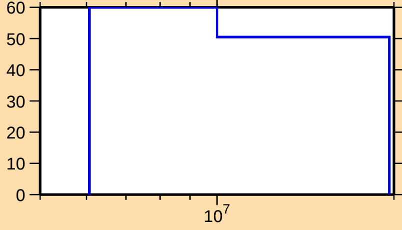
\Delta\sigma/\sigma vs. E for ^{127}\text{Sn}(n,n_1)
