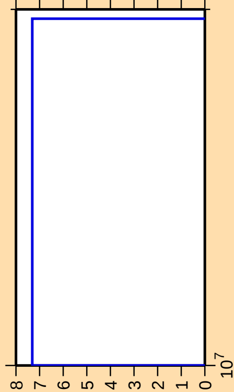
\Delta\sigma/\sigma vs. E for ^{127}\text{Sn}(n,\text{nd})
