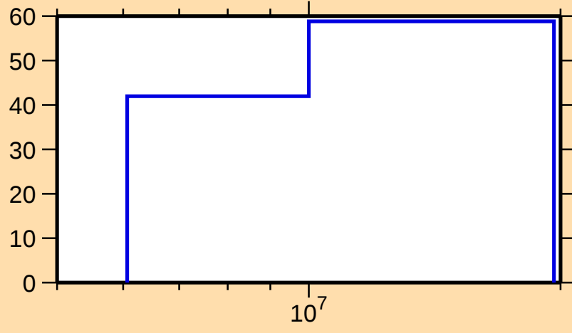
\Delta\sigma/\sigma vs. E for ^{127}\text{Sn}(n,n\text{cont.})
