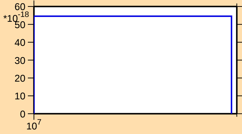
\sigma vs. E for ^{127}\text{Sn}(n,2np)
