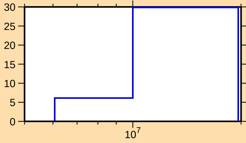
\Delta\sigma/\sigma vs. E for ^{127}\text{Sn}(n,\text{ncont.})
