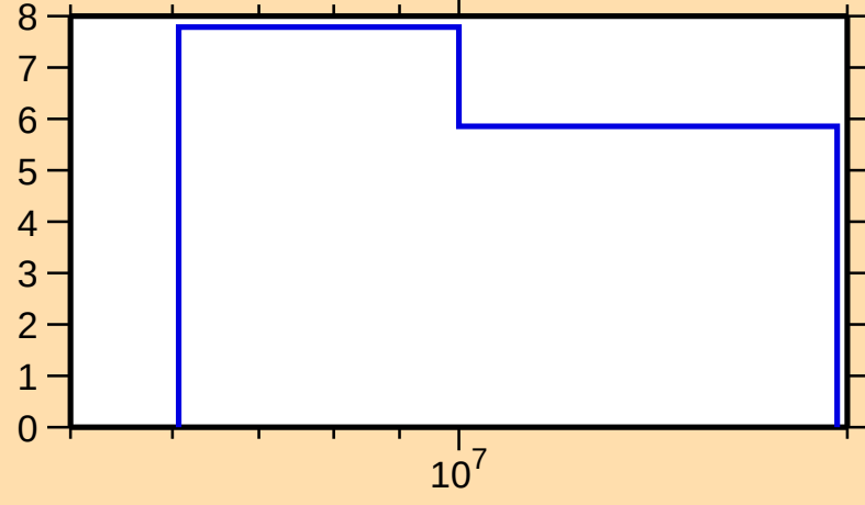
\Delta\sigma/\sigma vs. E for ^{127}\text{Sn}(n,2n)
