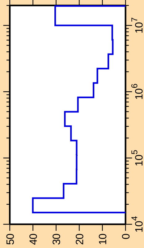
\Delta\sigma/\sigma vs. E for ^{127}\text{Sn}(n,\text{inel.})
