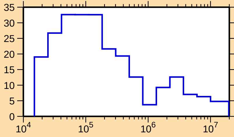
\Delta\sigma/\sigma vs. E for ^{127}\text{Sn}(n,\text{el.})
