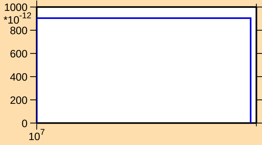
\sigma vs. E for ^{127}\text{Sn}(n,n\alpha)
