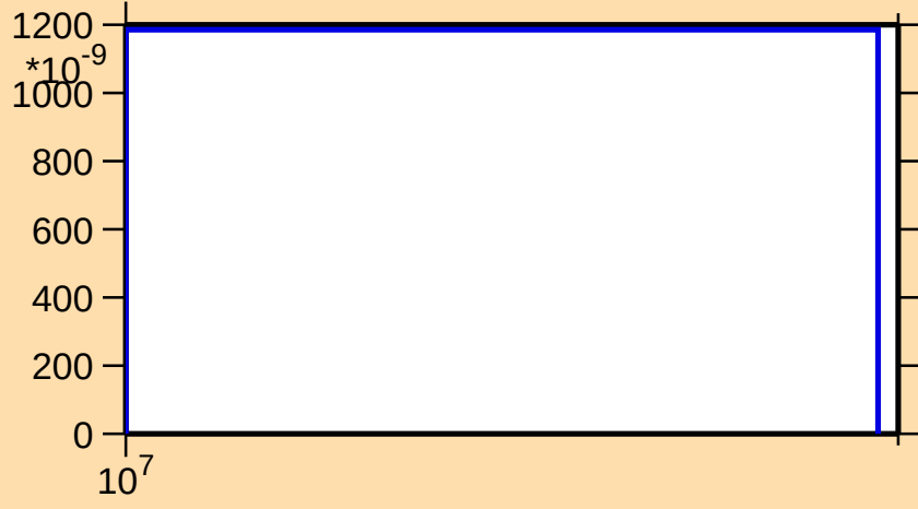
\sigma vs. E for ^{127}\text{Sn}(n,d)
