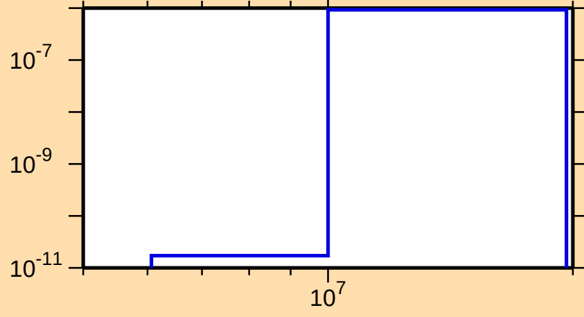
\sigma vs. E for ^{127}\text{Sn}(n,\alpha)
