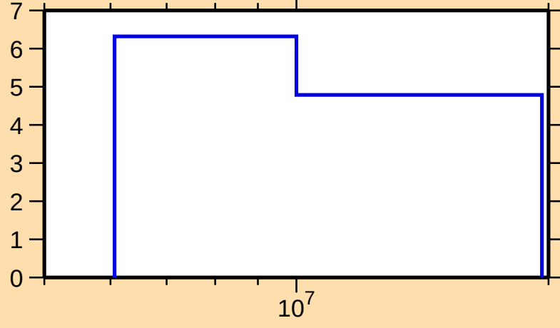
\Delta\sigma/\sigma vs. E for ^{127}\text{Sn}(n,\text{el.})
