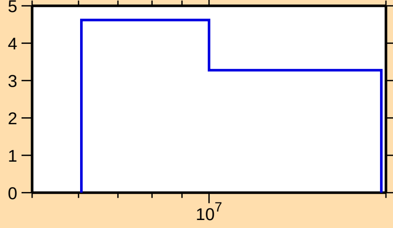
\Delta\sigma/\sigma vs. E for ^{127}\text{Sn}(n,\text{nonel.})
