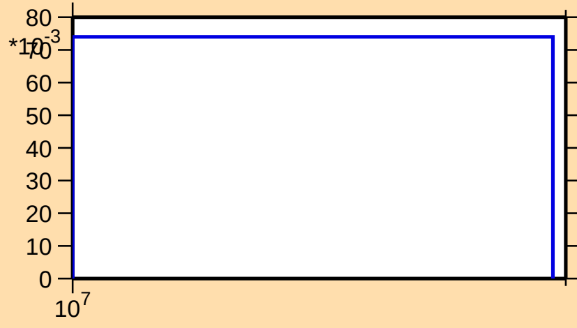
\sigma vs. E for ^{127}\text{Sn}(n,3n)
