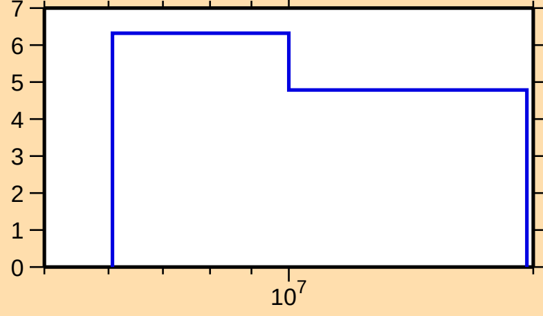
\Delta\sigma/\sigma vs. E for ^{127}\text{Sn}(n,\text{el.})
