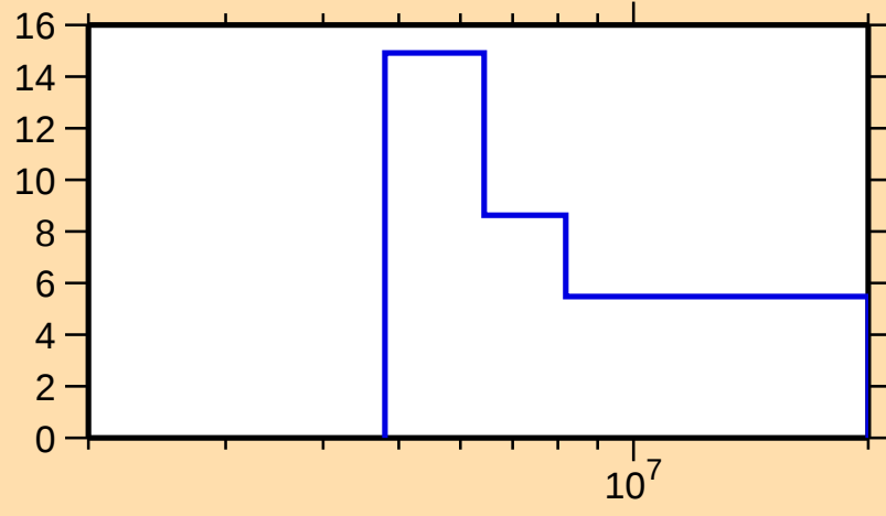
\Delta\sigma/\sigma vs. E for ^{127}\text{Sn}(n,2n)
