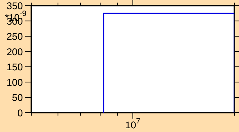
\sigma vs. E for ^{127}\text{Sn}(n,np)
