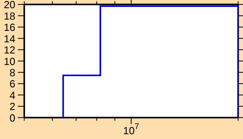
\Delta\sigma/\sigma vs. E for ^{127}\text{Sn}(n,n\text{cont.})
