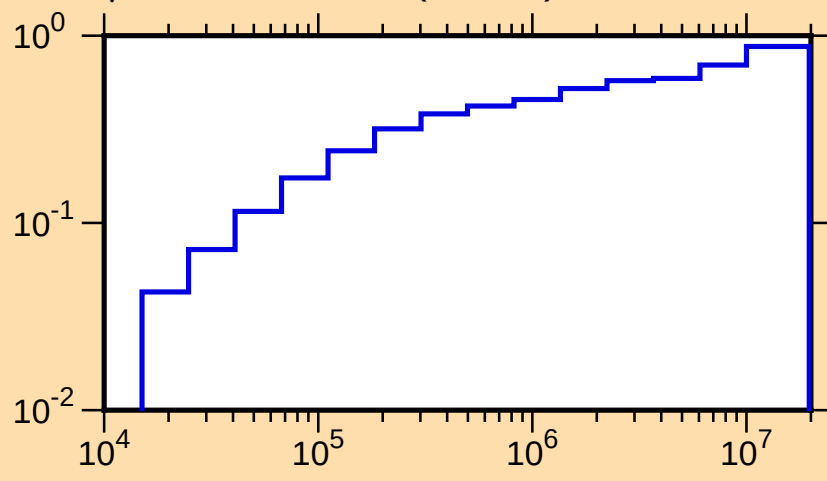
\mu vs. E for ^{129}\text{Sn}(\text{mt251})
