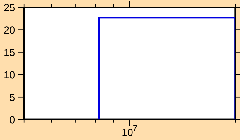
\Delta\sigma/\sigma vs. E for ^{129}\text{Sn}(n,\text{ncont.})
