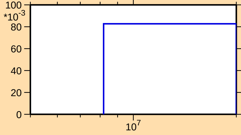
\sigma vs. E for ^{129}\text{Sn}(n,3n)
