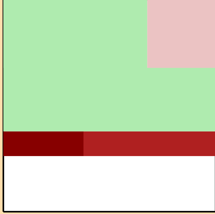
\Delta\sigma/\sigma vs. E for ^{82}\text{Sr}(n,\text{nonel.})
