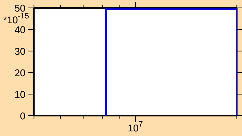
\sigma vs. E for ^{82}\text{Sr}(\text{mt } 45)
