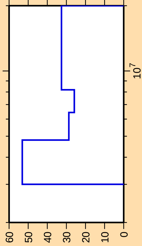
\Delta\sigma/\sigma vs. E for ^{82}\text{Sr}(\text{n},\text{ncont.})
