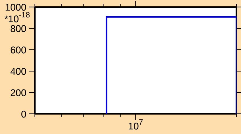
\sigma vs. E for ^{82}\text{Sr}(n,2np)
