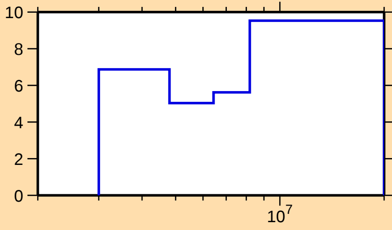
\Delta\sigma/\sigma vs. E for ^{82}\text{Sr}(\text{n},\text{tot.})
