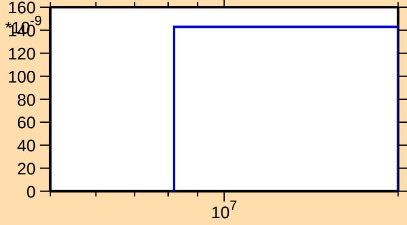
\sigma vs. E for ^{82}\text{Sr}(n,\text{pd})
