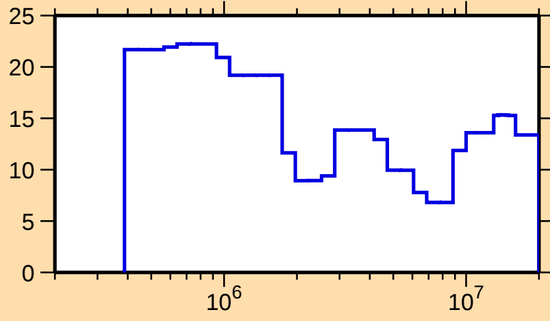
\Delta\sigma/\sigma vs. E for ^{87}\text{Sr}(n,\text{el.})
