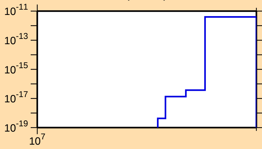
\sigma vs. E for ^{87}\text{Sr}(n,2n\alpha)
