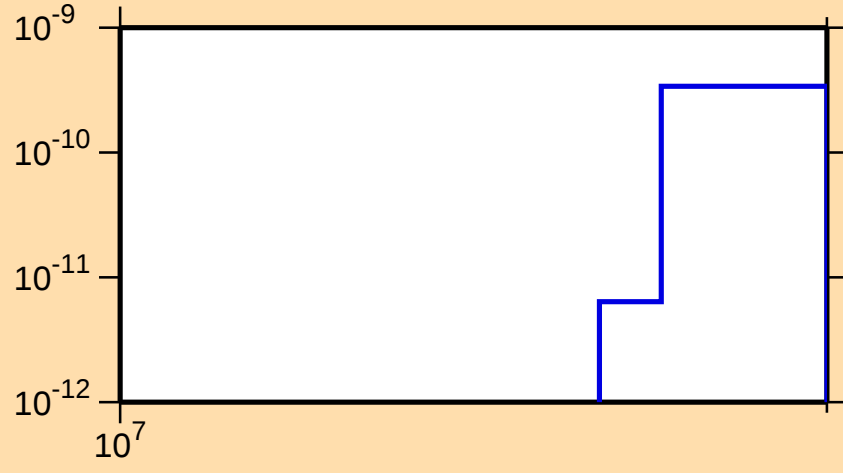
\sigma vs. E for ^{87}\text{Sr}(n,p\alpha)
