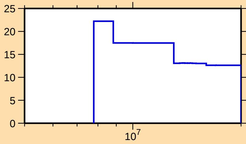
\Delta\sigma/\sigma vs. E for ^{87}\text{Sr}(n,2n)
