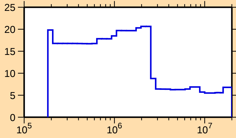
\Delta\sigma/\sigma vs. E for ^{87}\text{Sr}(n,\text{nonel.})
