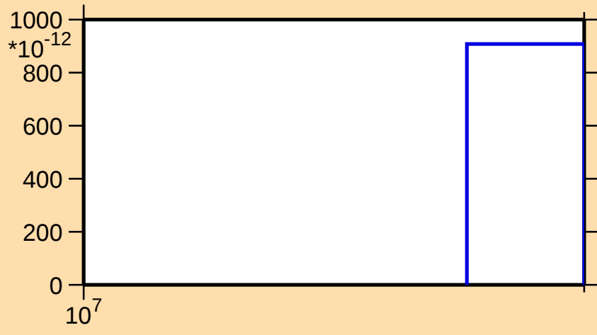
\sigma vs. E for ^{87}\text{Sr}(n,2np)
