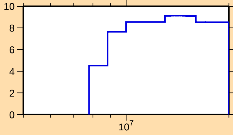
\Delta\sigma/\sigma vs. E for ^{87}\text{Sr}(n,\text{tot.})
