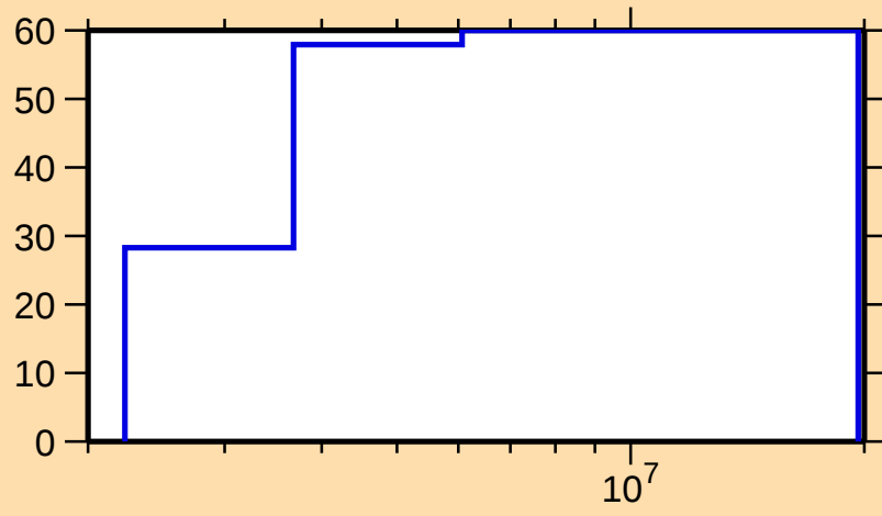
\Delta\sigma/\sigma vs. E for ^{87}\text{Sr}(n,n_1)
