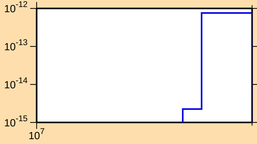
\sigma vs. E for ^{89}\text{Sr}(n,p\alpha)
