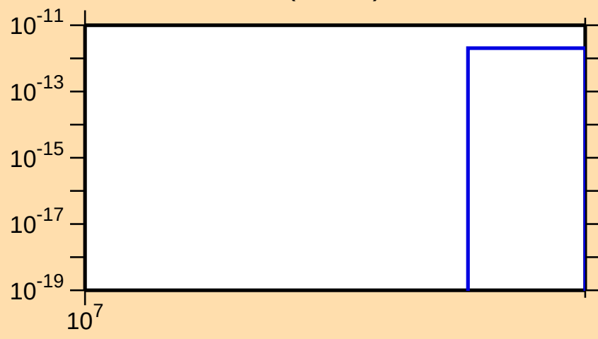
\sigma vs. E for ^{89}\text{Sr}(n,2n\alpha)
