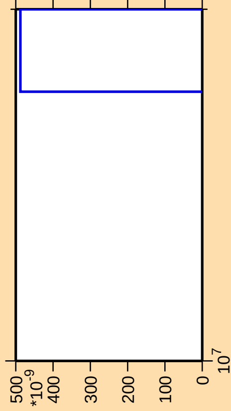
\Delta\sigma/\sigma vs. E for ^{89}\text{Sr} (mt 34)
