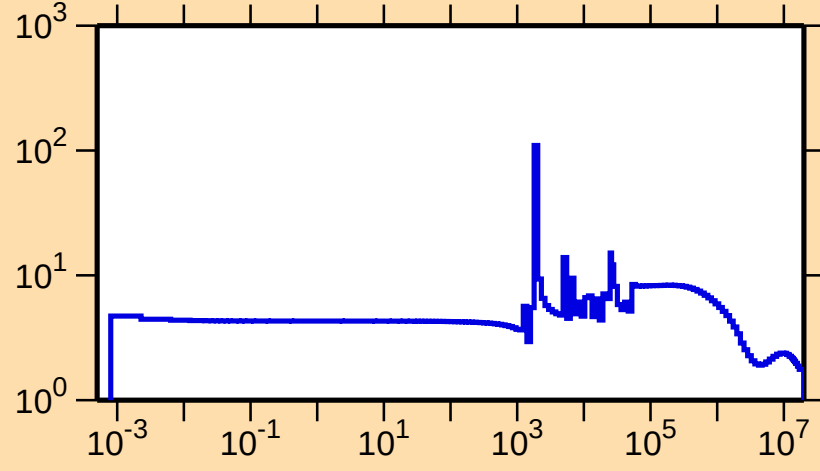
\sigma vs. E for ^{89}\text{Sr}(n,\text{el.})
