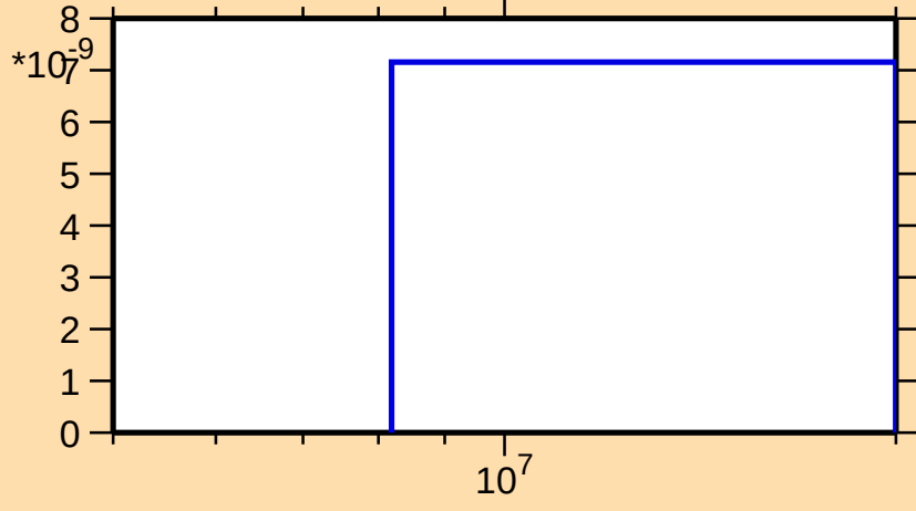
\sigma vs. E for ^{89}\text{Sr}(n,\text{nd})
