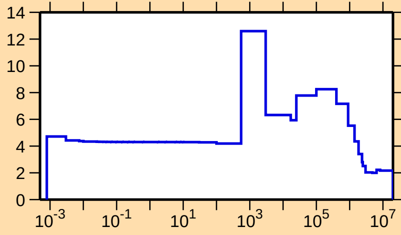
\sigma vs. E for ^{89}\text{Sr}(n,\text{el.})
