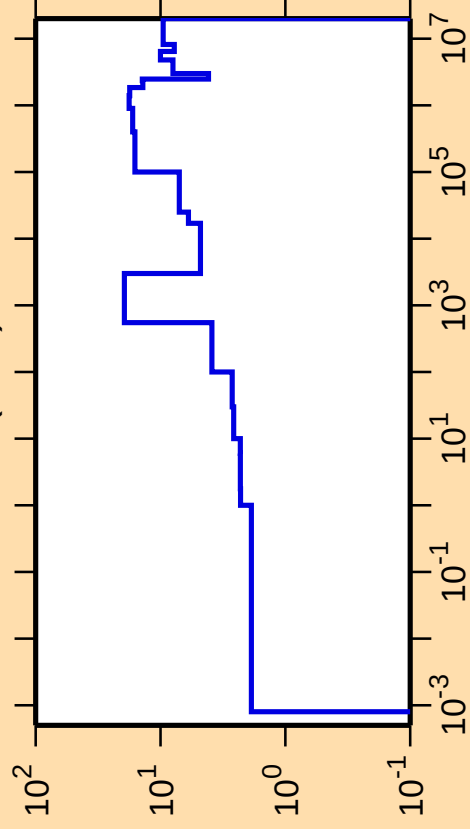
\Delta\sigma/\sigma vs. E for ^{89}\text{Sr}(n,\text{el.})
