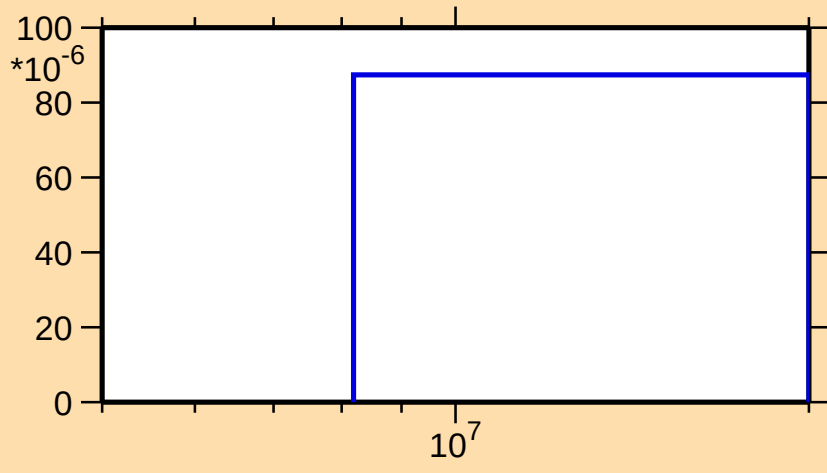
\sigma vs. E for ^{89}\text{Sr}(n,t)
