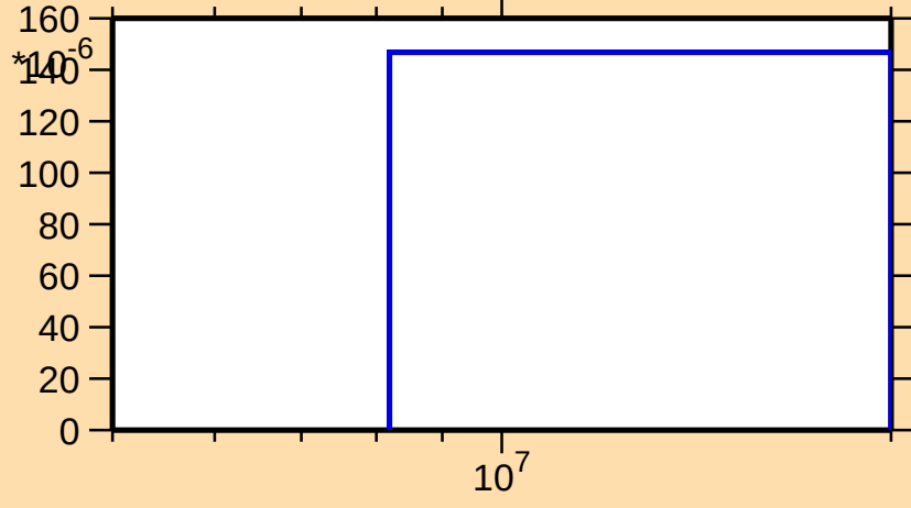
\sigma vs. E for ^{89}\text{Sr}(n,np)
