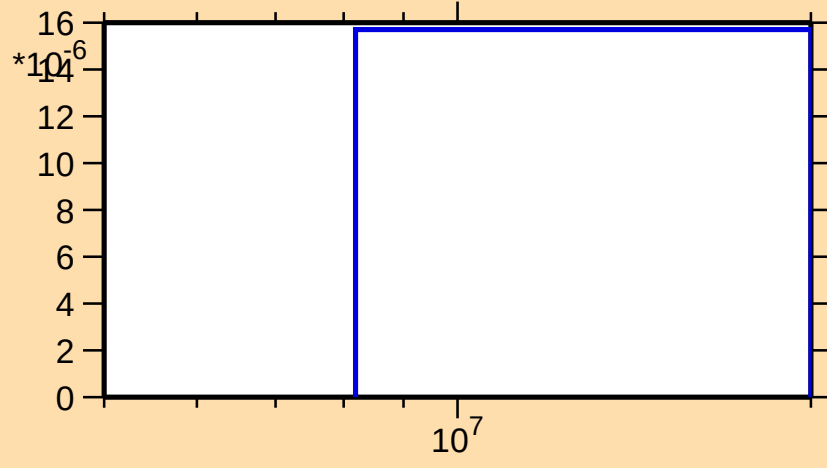
\sigma vs. E for ^{89}\text{Sr}(n,\alpha)
