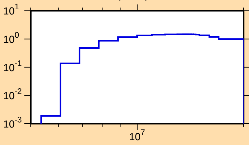
\sigma vs. E for ^{91}\text{Sr}(n,2n)
