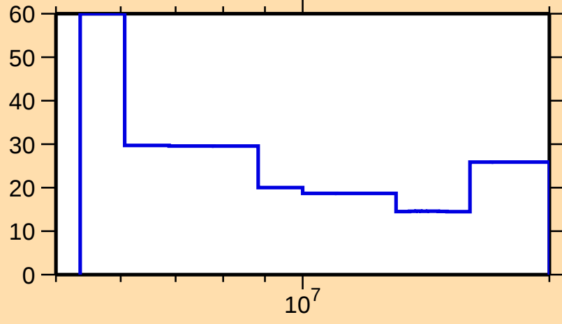
\Delta\sigma/\sigma vs. E for ^{91}\text{Sr}(n,2n)
