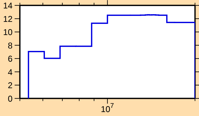
\Delta\sigma/\sigma vs. E for ^{91}\text{Sr}(n,\text{tot.})
