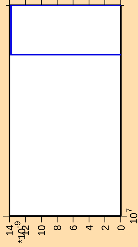
\Delta\sigma/\sigma vs. E for ^{91}\text{Sr} (mt 34)
