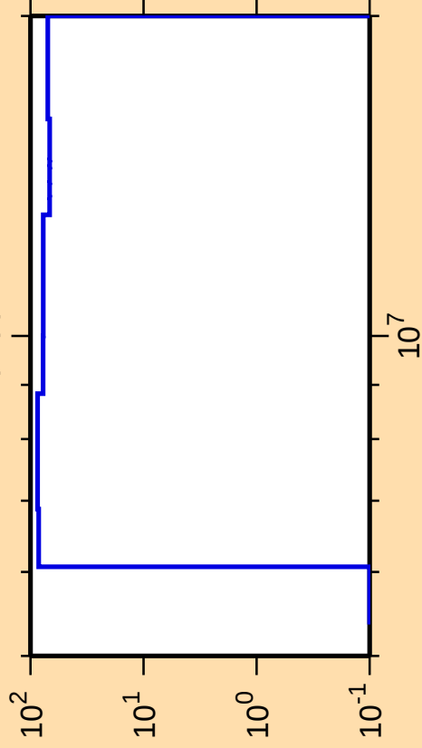
\Delta\sigma/\sigma vs. E for ^{91}\text{Sr}(n,p)
