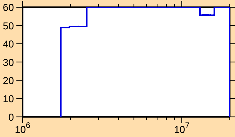
\Delta\sigma/\sigma vs. E for ^{91}\text{Sr}(n,\gamma)
