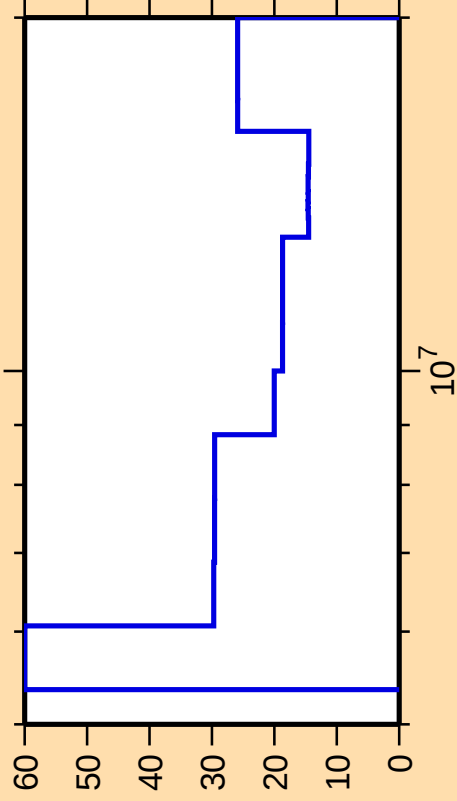
\Delta\sigma/\sigma vs. E for ^{91}\text{Sr}(n,2n)
