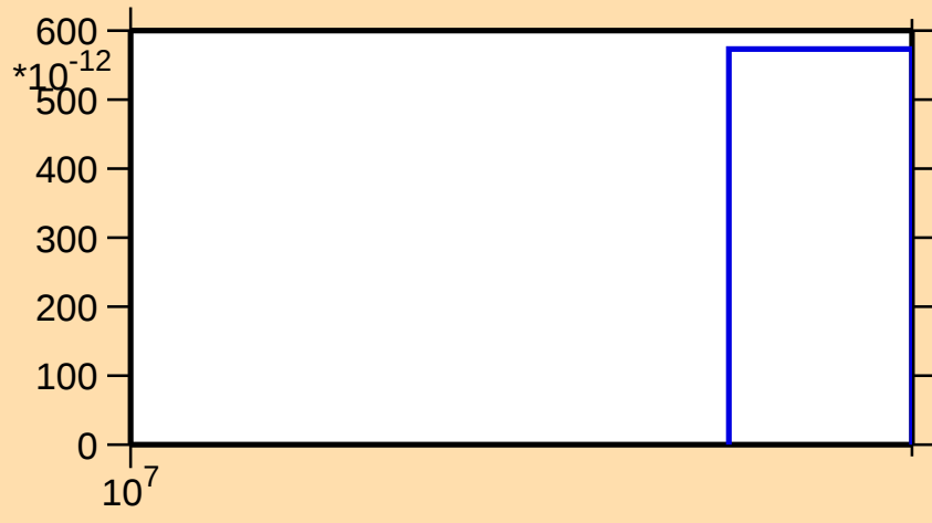
\sigma vs. E for ^{91}\text{Sr}(n,2np)
