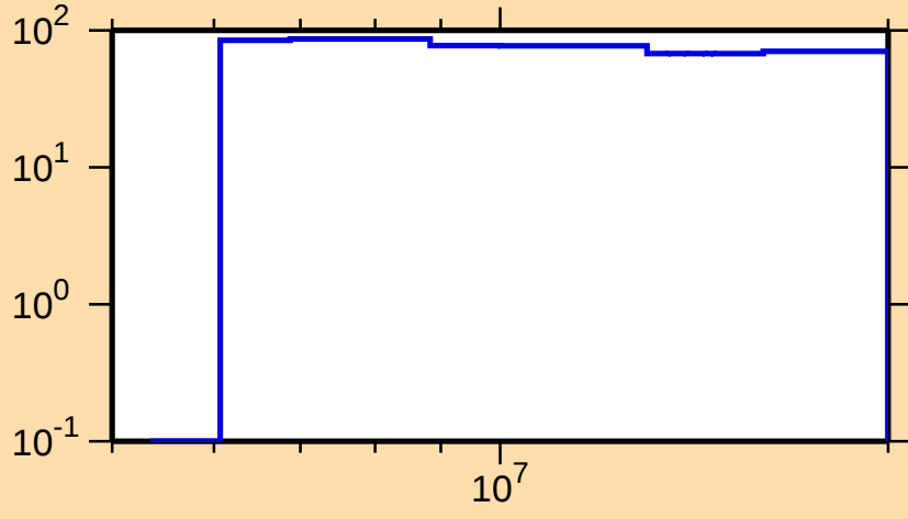
\Delta\sigma/\sigma vs. E for ^{91}\text{Sr}(n,p)
