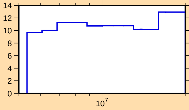
\Delta\sigma/\sigma vs. E for ^{91}\text{Sr}(n,\text{nonel.})
