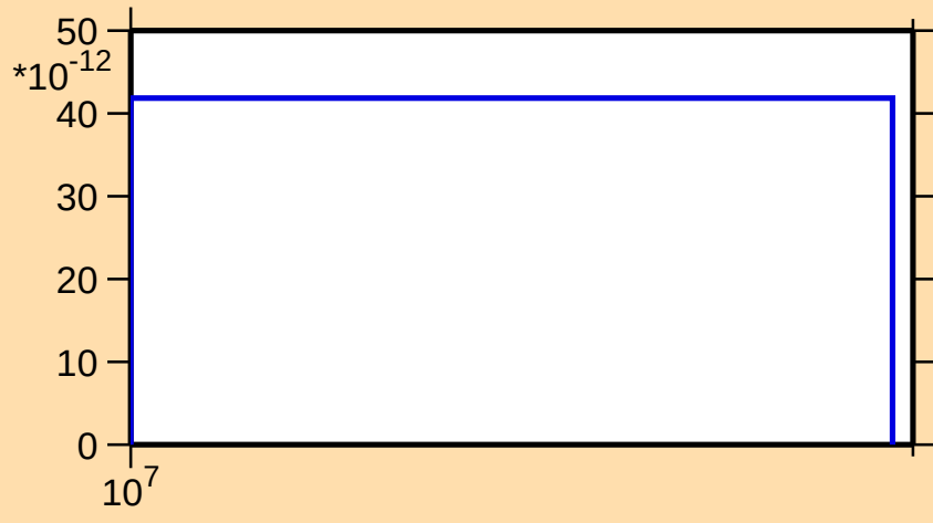
\sigma vs. E for ^{91}\text{Sr}(n,\text{nt})
