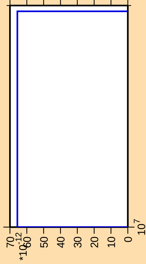
\Delta\sigma/\sigma vs. E for ^{91}\text{Sr} (mt 34)
