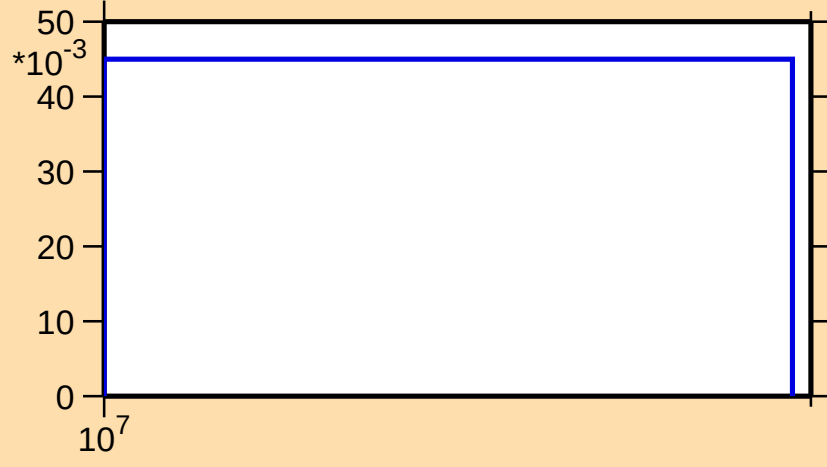
\sigma vs. E for ^{91}\text{Sr}(n,3n)
