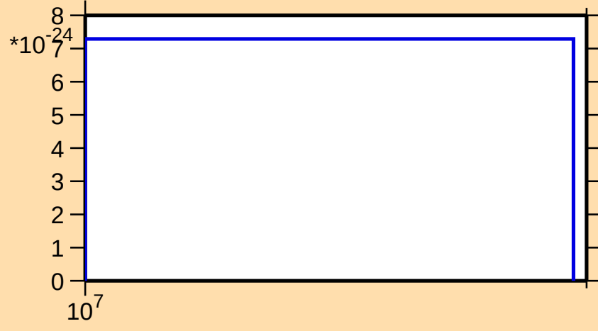
\sigma vs. E for ^{91}\text{Sr} (mt 34)
