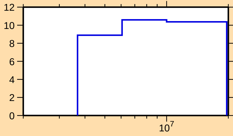
\Delta\sigma/\sigma vs. E for ^{91}\text{Sr}(\text{n},\text{nonel.})
