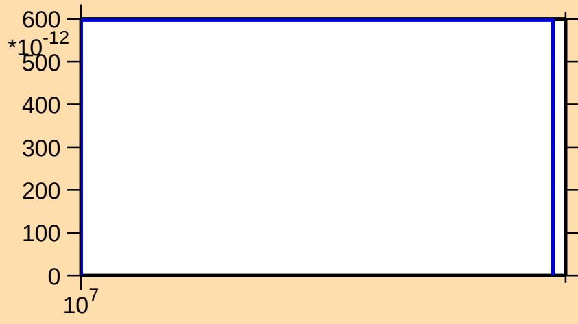
\sigma vs. E for ^{91}\text{Sr}(n,2n\alpha)
