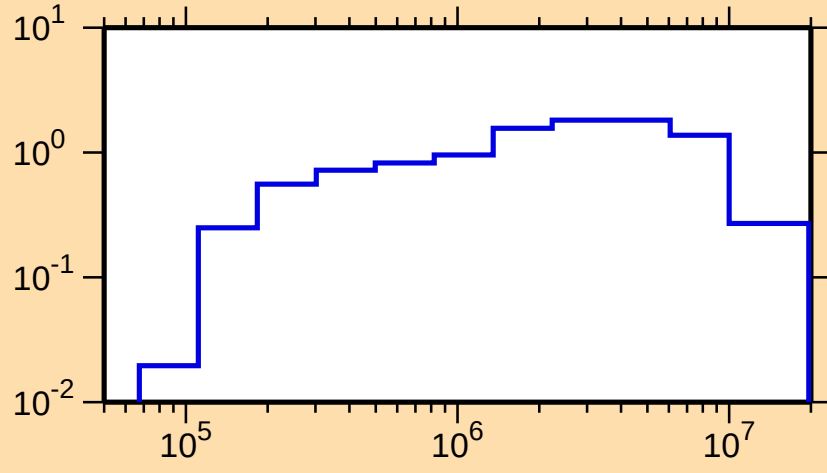
\sigma vs. E for ^{91}\text{Sr}(n,\text{inel.})
