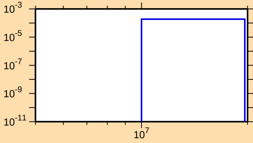
\sigma vs. E for ^{91}\text{Sr}(n,d)
