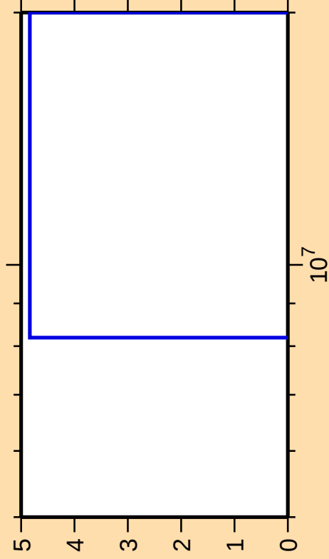
\Delta\sigma/\sigma vs. E for ^{91}\text{Sr}(n,2np)
