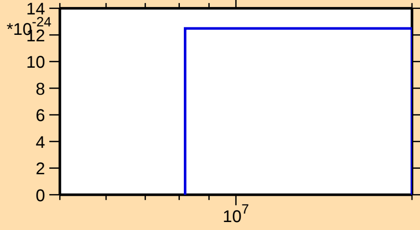
\sigma vs. E for ^{91}\text{Sr}(\text{mt } 34)
