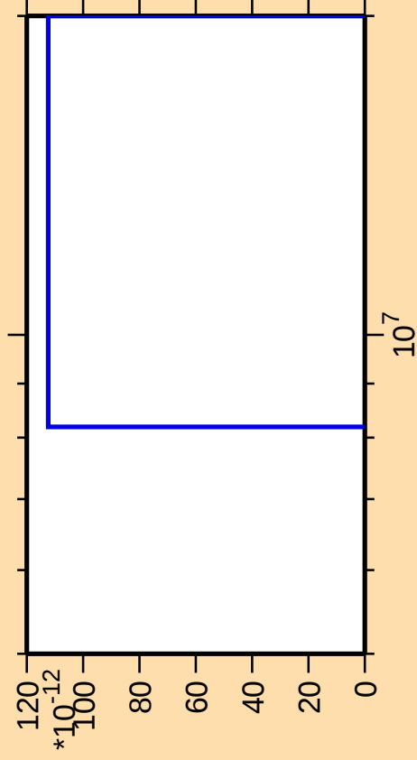
\Delta\sigma/\sigma vs. E for ^{91}\text{Sr}(\text{mt } 34)
