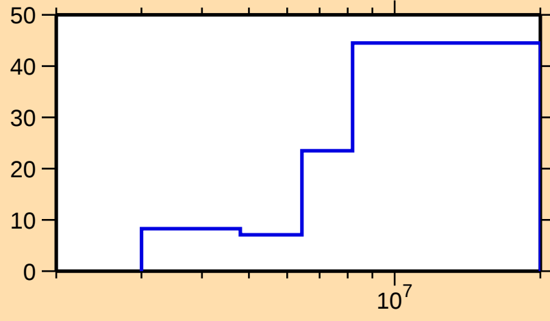
\Delta\sigma/\sigma vs. E for ^{91}\text{Sr}(\text{n},\text{inel.})
