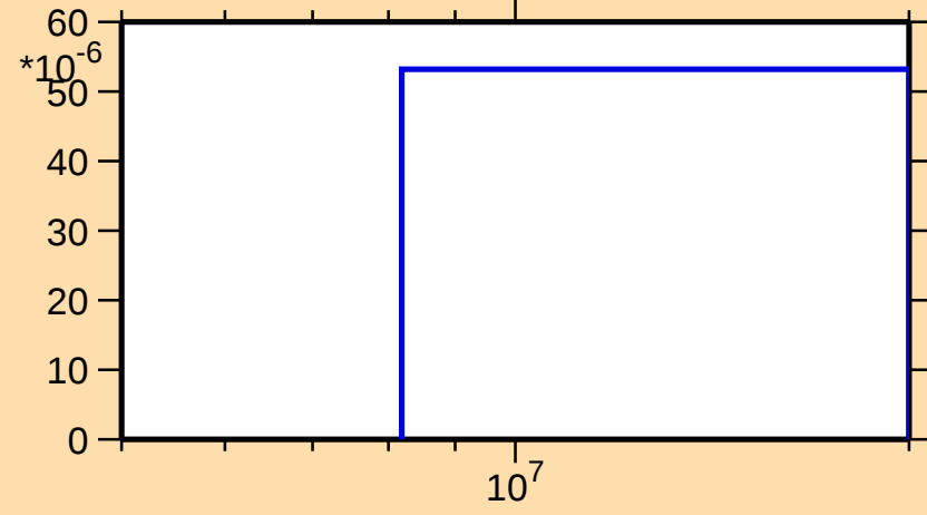
\sigma vs. E for ^{91}\text{Sr}(n,\alpha)
