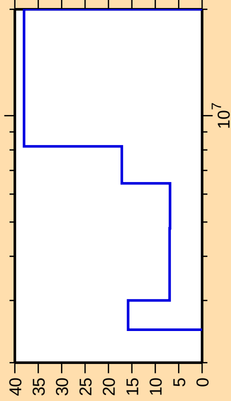
\Delta\sigma/\sigma vs. E for ^{93}\text{Sr}(\text{n},\text{ncont.})
