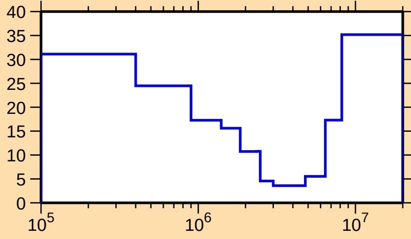
\Delta\sigma/\sigma vs. E for ^{93}\text{Sr}(n,\text{inel.})
