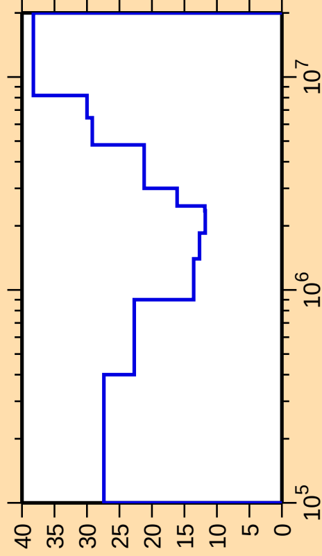
\Delta\sigma/\sigma vs. E for ^{93}\text{Sr}(n,n_1)
