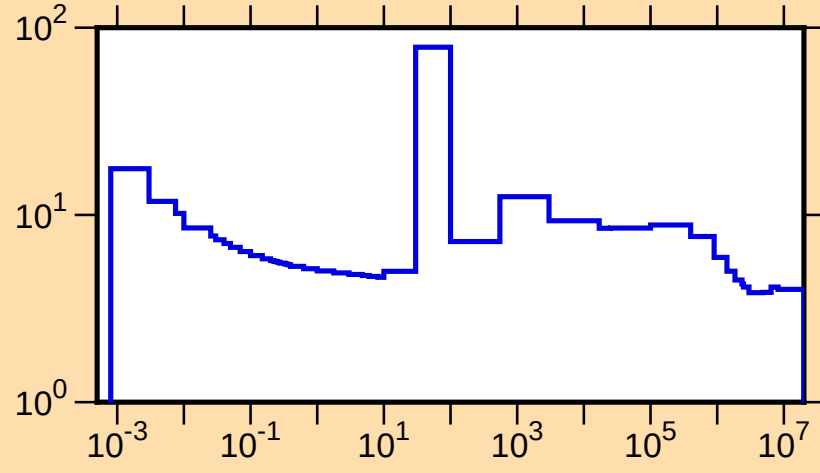
\sigma vs. E for ^{93}\text{Sr}(n,\text{tot.})
