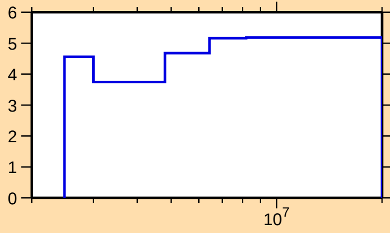
\Delta\sigma/\sigma vs. E for ^{93}\text{Sr}(\text{n},\text{nonel.})
