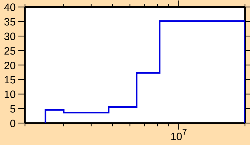
\Delta\sigma/\sigma vs. E for ^{93}\text{Sr}(\text{n},\text{inel.})
