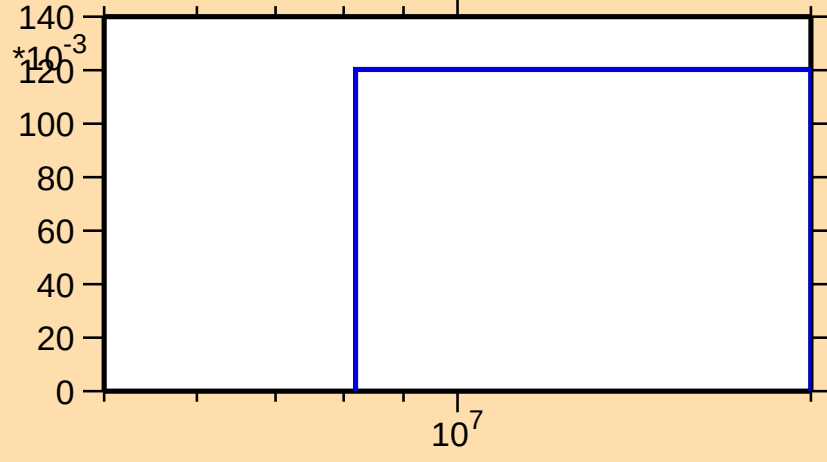
\sigma vs. E for ^{93}\text{Sr}(n,3n)
