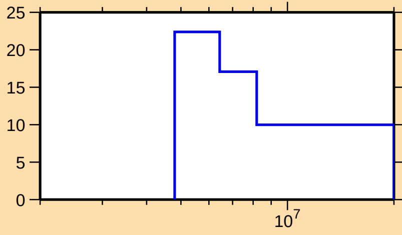
\Delta\sigma/\sigma vs. E for ^{93}\text{Sr}(n,2n)
