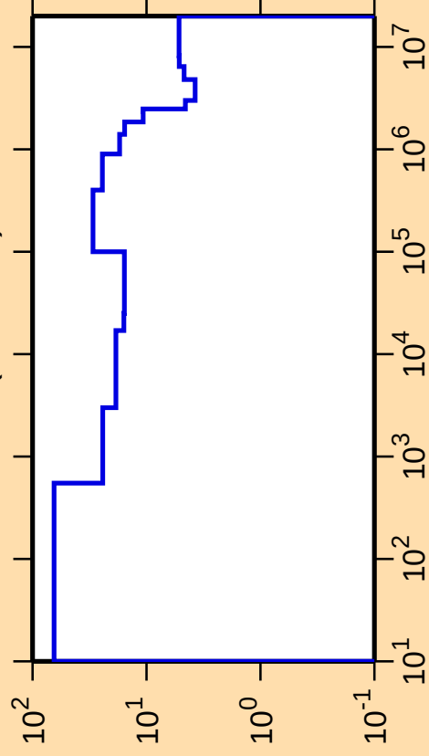
\Delta\sigma/\sigma vs. E for ^{93}\text{Sr}(n,\text{nonel.})
