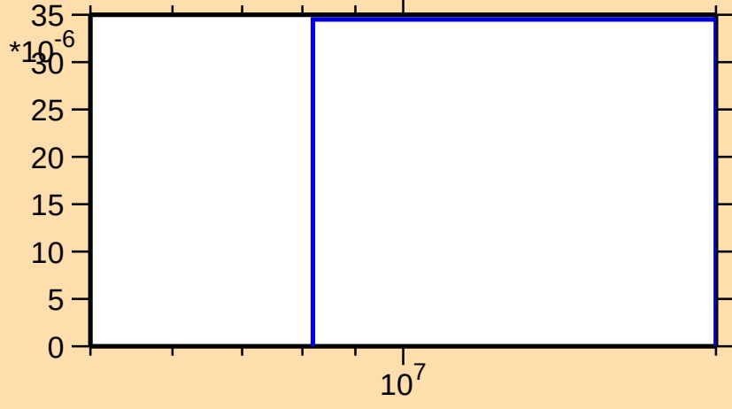
\sigma vs. E for ^{93}\text{Sr}(n,d)
