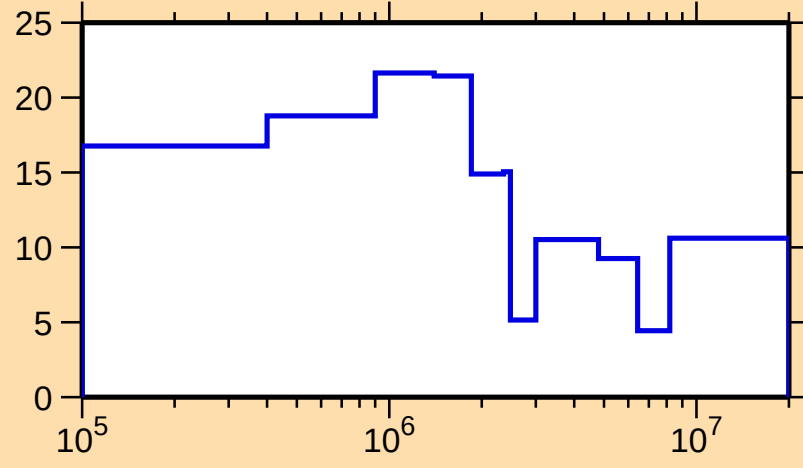
\Delta\sigma/\sigma vs. E for ^{93}\text{Sr}(n,\text{el.})
