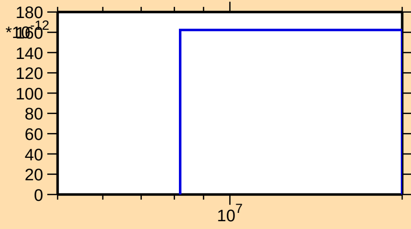
\sigma vs. E for ^{93}\text{Sr}(n,\text{nt})
