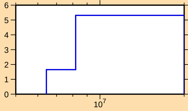
\Delta\sigma/\sigma vs. E for ^{93}\text{Sr}(n,\text{tot.})
