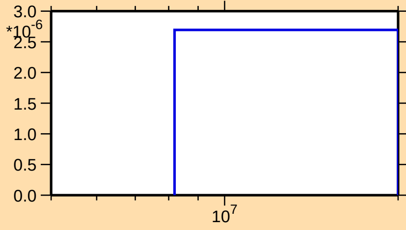
\sigma vs. E for ^{93}\text{Sr}(n,np)
