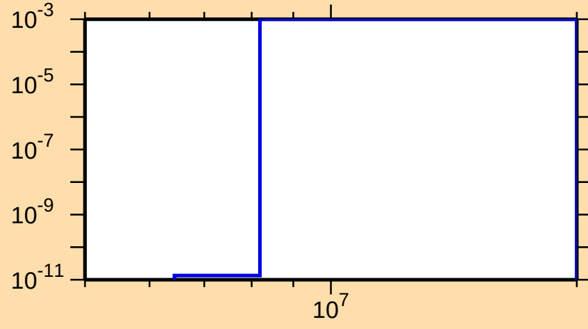
\sigma vs. E for ^{93}\text{Sr}(n,p)
