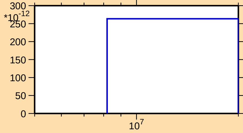
\sigma vs. E for ^{93}\text{Sr}(n,2n\alpha)
