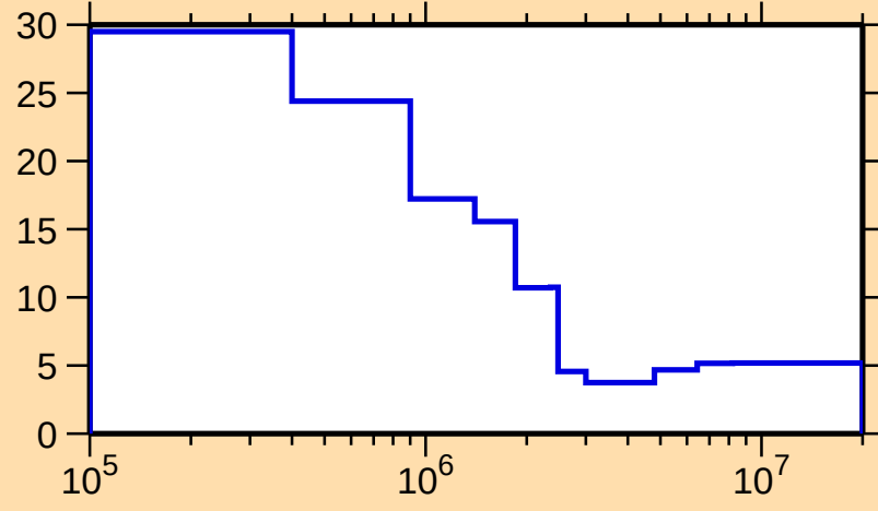
\Delta\sigma/\sigma vs. E for ^{93}\text{Sr}(n,\text{nonel.})
