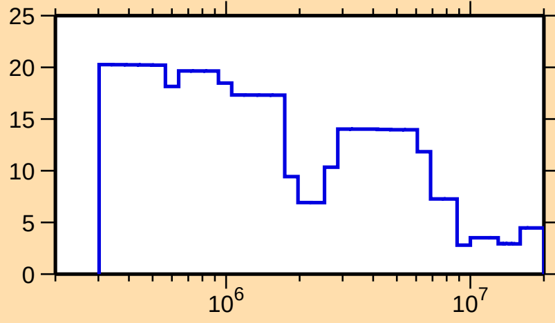
\Delta\sigma/\sigma vs. E for ^{160}\text{Ta}(n,\text{tot.})
