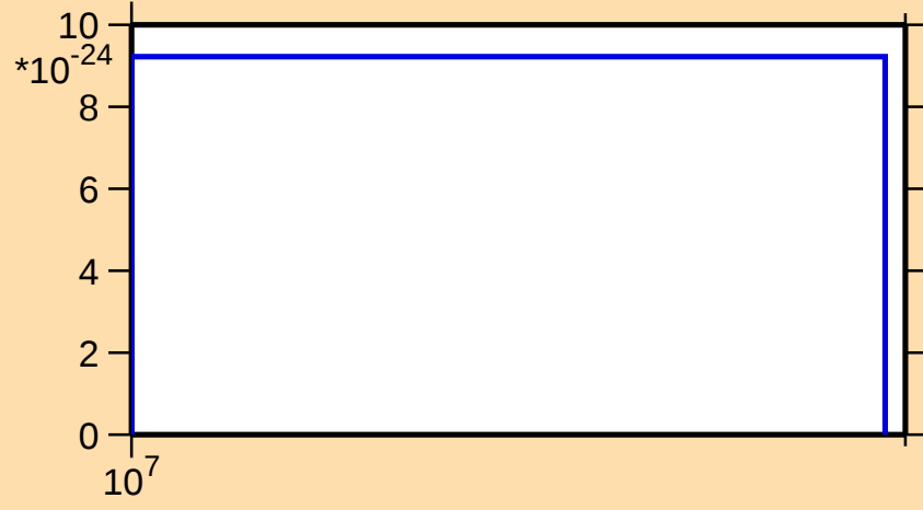
\sigma vs. E for ^{160}\text{Ta}(\text{mt } 11)
