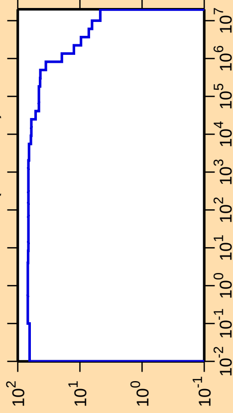
\Delta\sigma/\sigma vs. E for ^{160}\text{Ta}(n,\text{nonel.})
