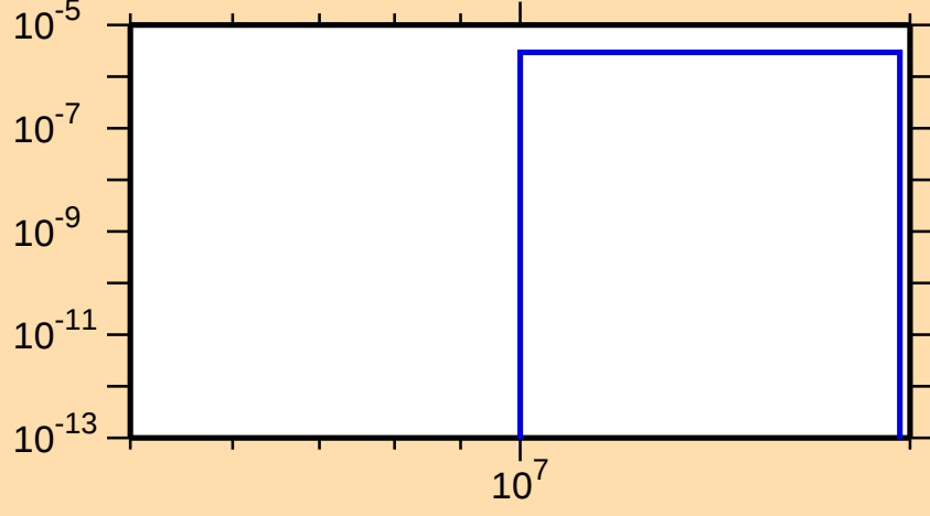
\sigma vs. E for ^{160}\text{Ta}(n,\text{pt})
