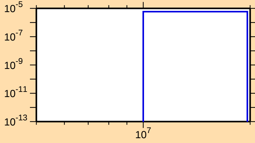
\sigma vs. E for ^{160}\text{Ta}(n,\text{nd})
