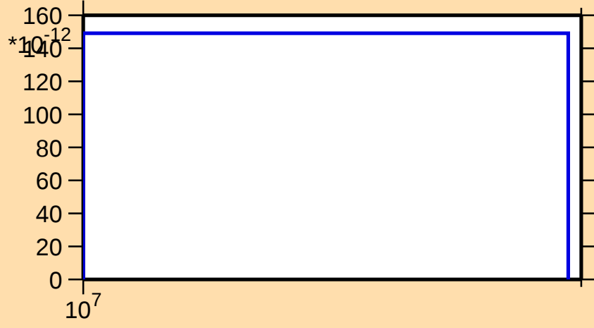
\sigma vs. E for ^{160}\text{Ta}(n,\text{nt})
