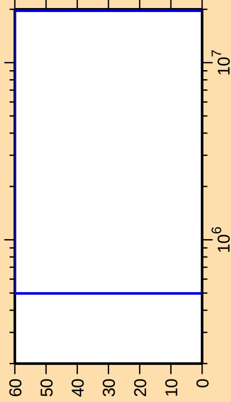
\Delta\sigma/\sigma vs. E for ^{160}\text{Ta}(n,\alpha)
