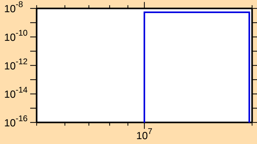
\sigma vs. E for ^{160}\text{Ta}(\text{mt } 34)
