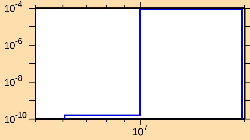
\sigma vs. E for ^{160}\text{Ta}(n,\text{pd})
