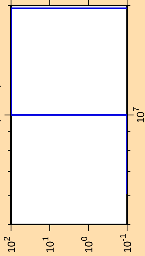
\Delta\sigma/\sigma vs. E for ^{160}\text{Ta}(\text{mt } 34)
