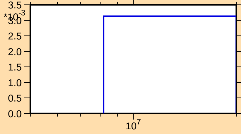
\sigma vs. E for ^{160}\text{Ta}(n,2np)
