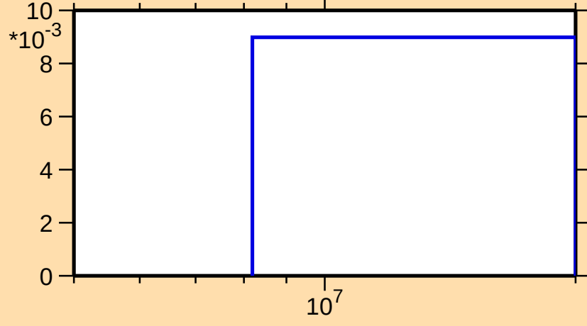
\sigma vs. E for ^{160}\text{Ta}(n,2n)
