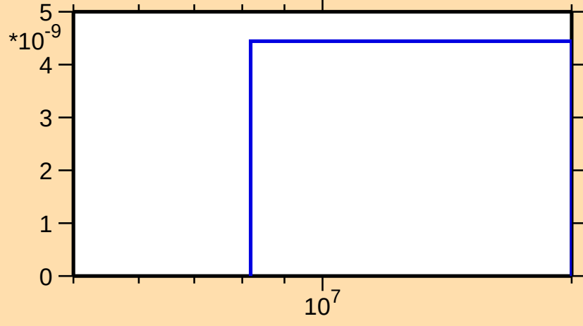
\sigma vs. E for ^{160}\text{Ta}(\text{mt } 34)
