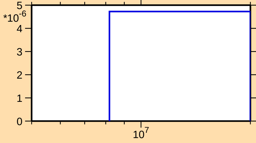
\sigma vs. E for ^{160}\text{Ta}(n,\text{nd})
