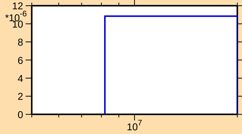
\sigma vs. E for ^{160}\text{Ta}(n,2n\alpha)
