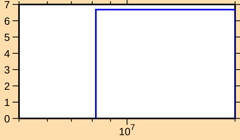
\Delta\sigma/\sigma vs. E for ^{160}\text{Ta}(n,\text{el.})
