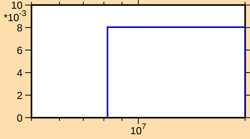
\sigma vs. E for ^{162}\text{Ta}(n,2np)
