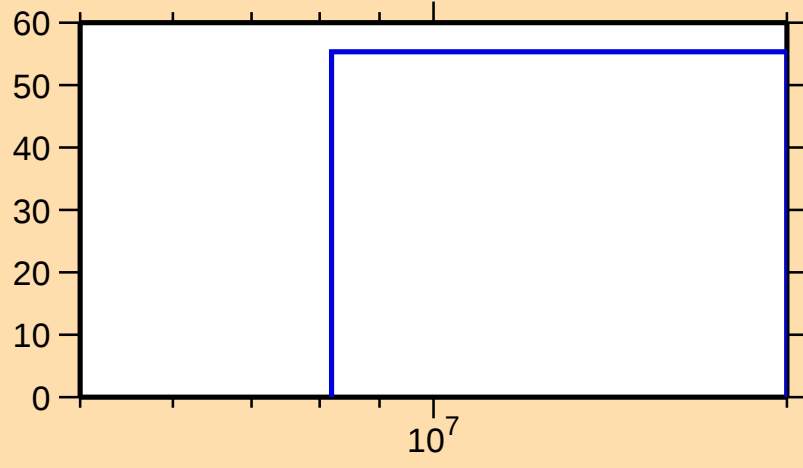
\Delta\sigma/\sigma vs. E for ^{162}\text{Ta}(n,\text{inel.})
