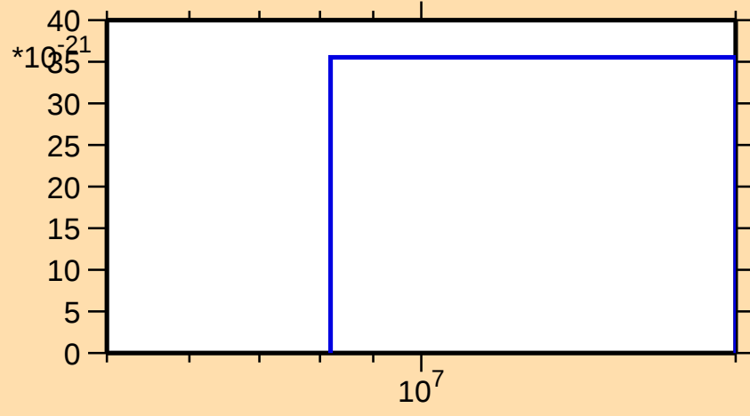
\sigma vs. E for ^{162}\text{Ta}(\text{mt } 11)
