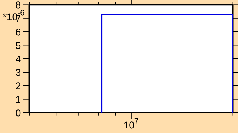
\sigma vs. E for ^{162}\text{Ta}(n,\text{nd})
