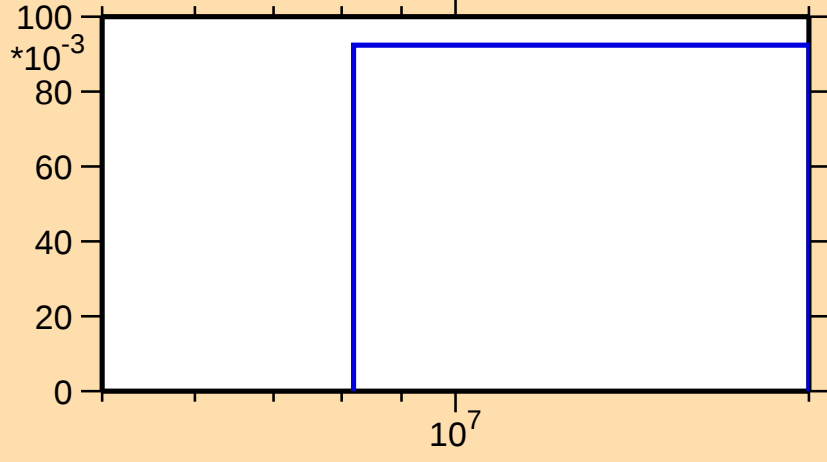
\sigma vs. E for ^{162}\text{Ta}(n,2n)
