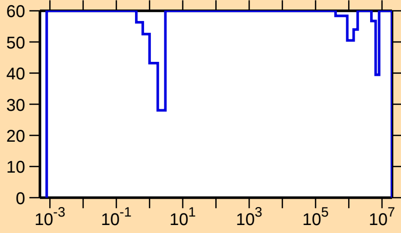
\Delta\sigma/\sigma vs. E for ^{162}\text{Ta}(n,\gamma)
