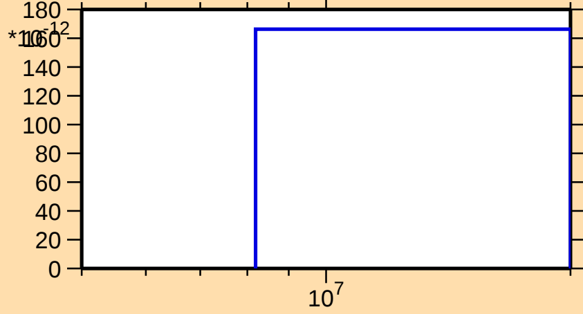
\sigma vs. E for ^{162}\text{Ta}(n,nt)
