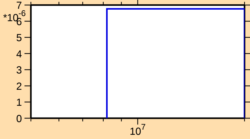
\sigma vs. E for ^{162}\text{Ta}(n,\text{pd})
