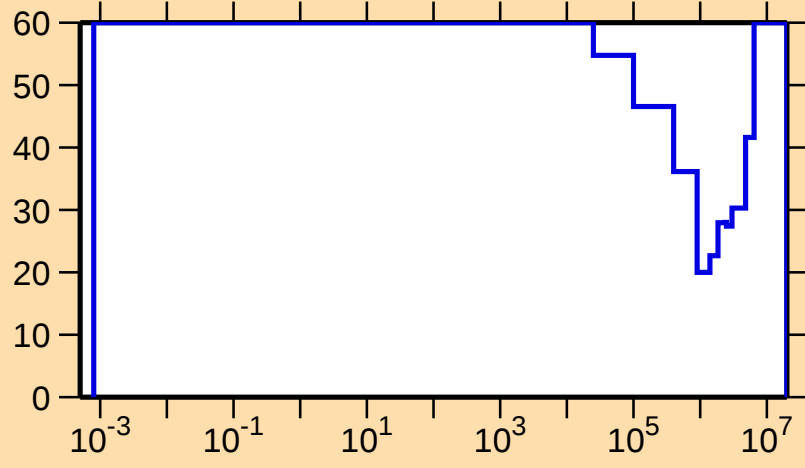
\Delta\sigma/\sigma vs. E for ^{162}\text{Ta}(n,p)
