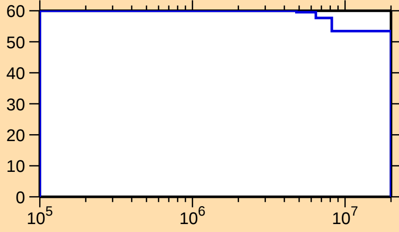
\Delta\sigma/\sigma vs. E for ^{162}\text{Ta}(n, n_1)
