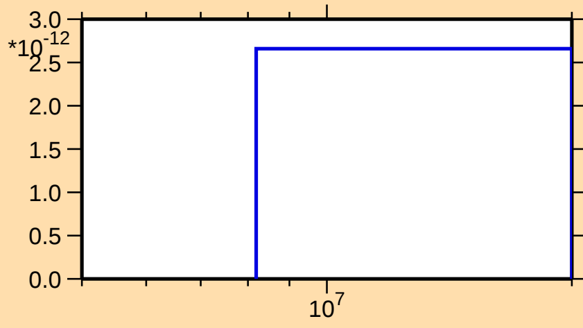
\sigma vs. E for ^{170}\text{Ta}(\text{mt } 34)
