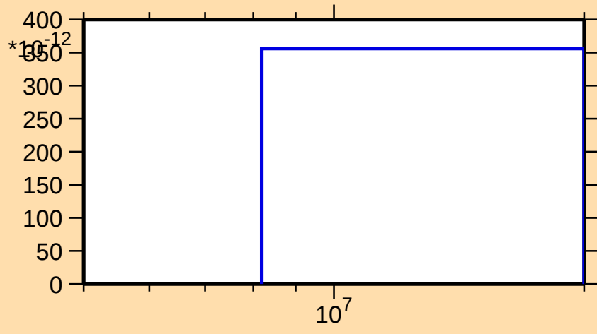
\sigma vs. E for ^{170}\text{Ta}(\text{mt117})
