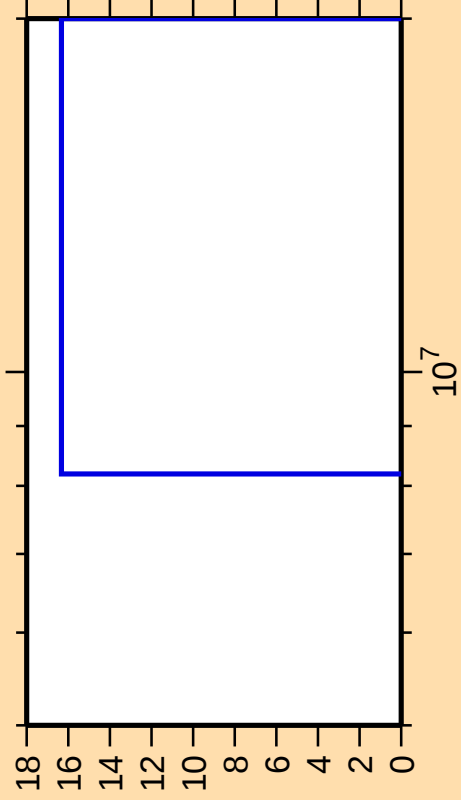
\Delta\sigma/\sigma vs. E for ^{170}\text{Ta}(\text{mt } 34)
