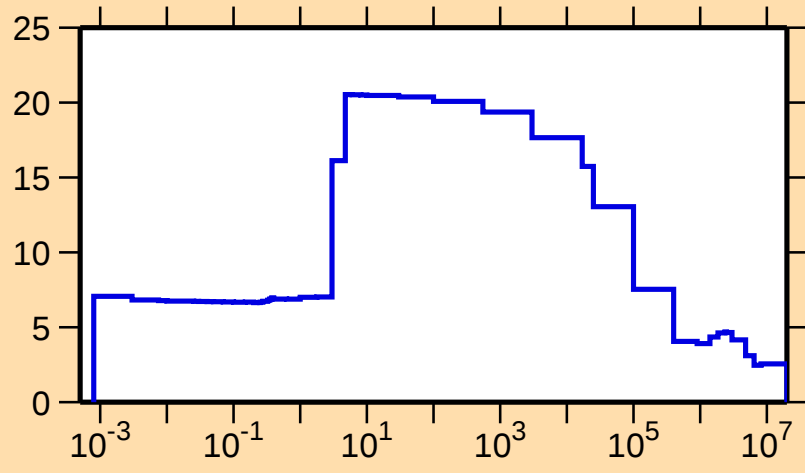
\sigma vs. E for ^{170}\text{Ta}(n,\text{el.})
