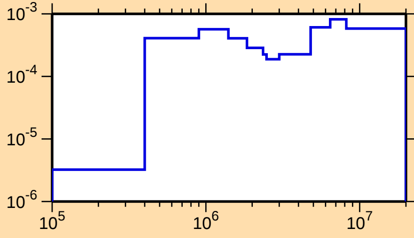
\sigma vs. E for ^{170}\text{Ta}(n,n_2)
