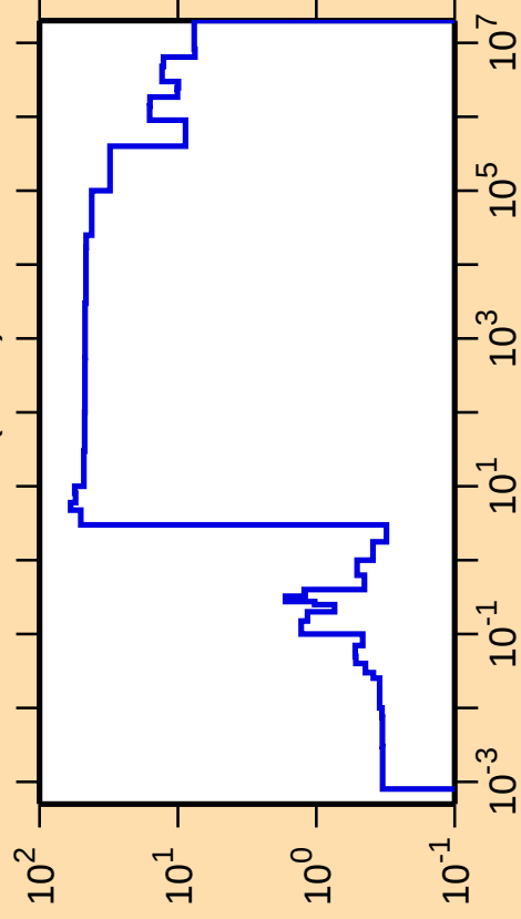
\Delta\sigma/\sigma vs. E for ^{170}\text{Ta}(n,\text{el.})
