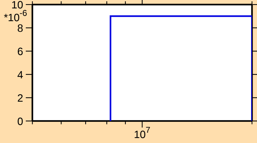
\sigma vs. E for ^{170}\text{Ta}(n,3n)
