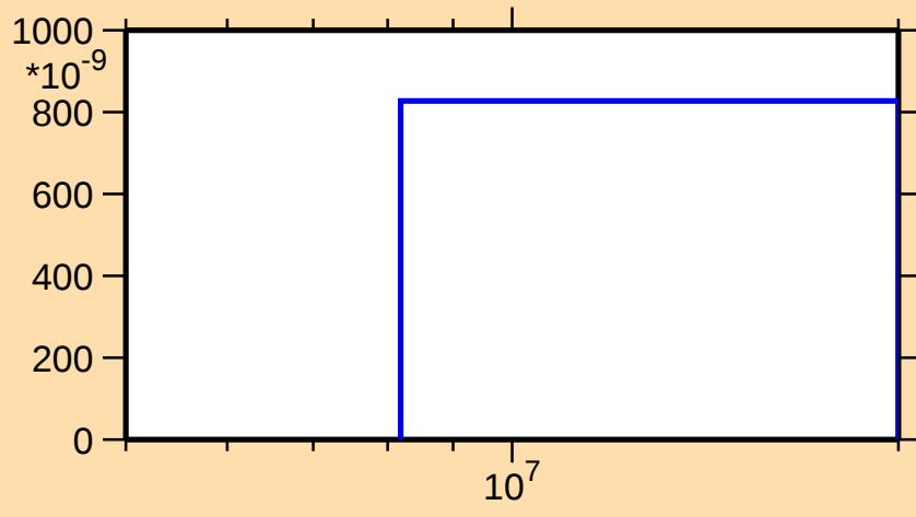
\sigma vs. E for ^{170}\text{Ta}(n,\text{He}3)
