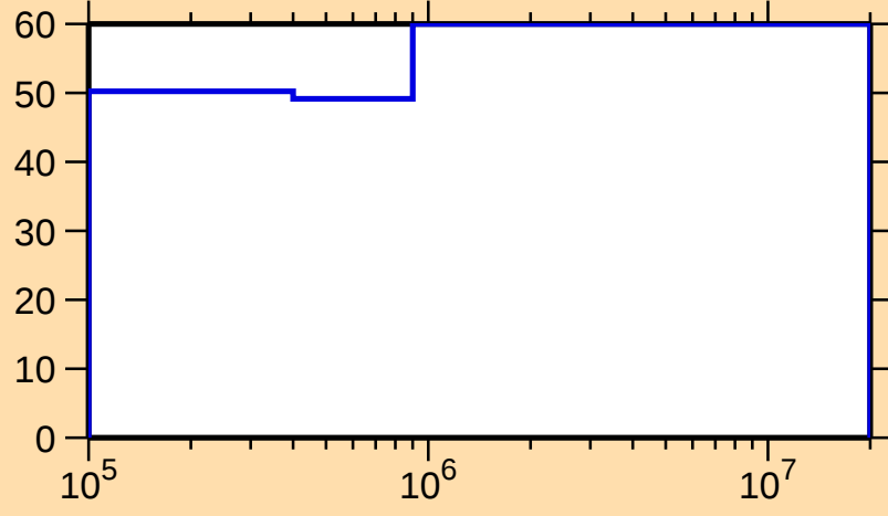
\Delta\sigma/\sigma vs. E for ^{170}\text{Ta}(n,n_1)
