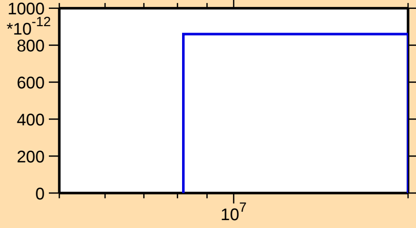
\sigma vs. E for ^{170}\text{Ta}(n,nt)
