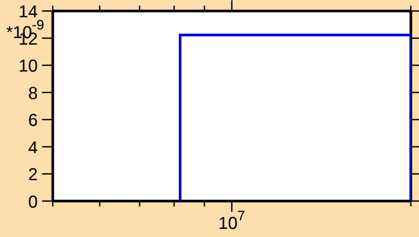
\sigma vs. E for ^{170}\text{Ta}(\text{mt } 45)
