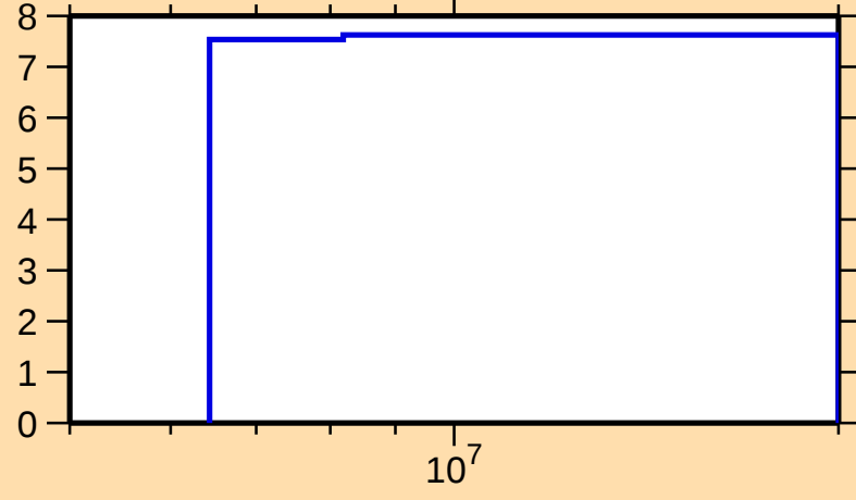
\Delta\sigma/\sigma vs. E for ^{170}\text{Ta}(n,\text{el.})
