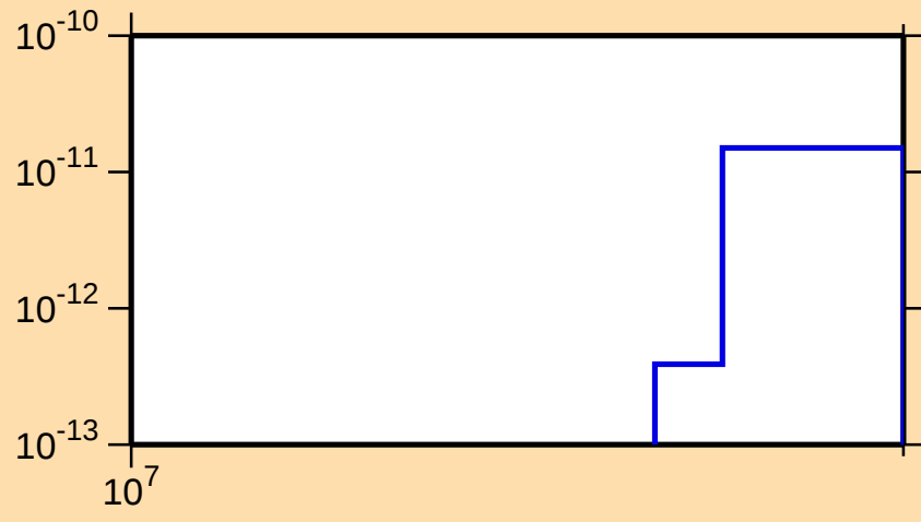
\sigma vs. E for ^{174}\text{Ta}(n,\text{pd})
