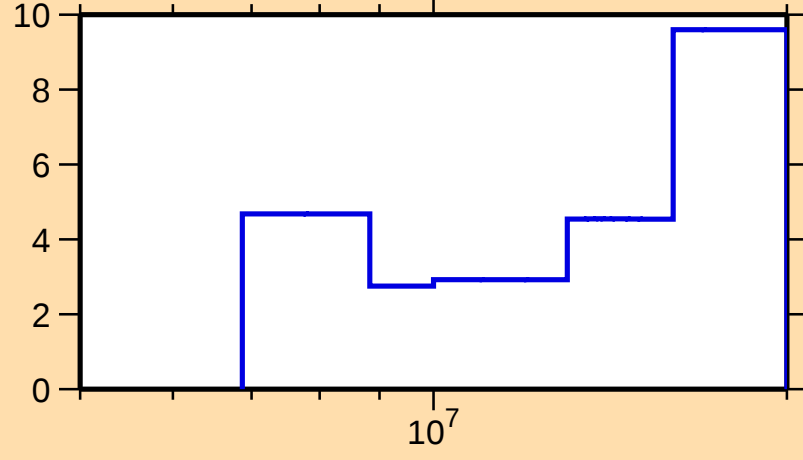
\Delta\sigma/\sigma vs. E for ^{174}\text{Ta}(n,\text{tot.})
