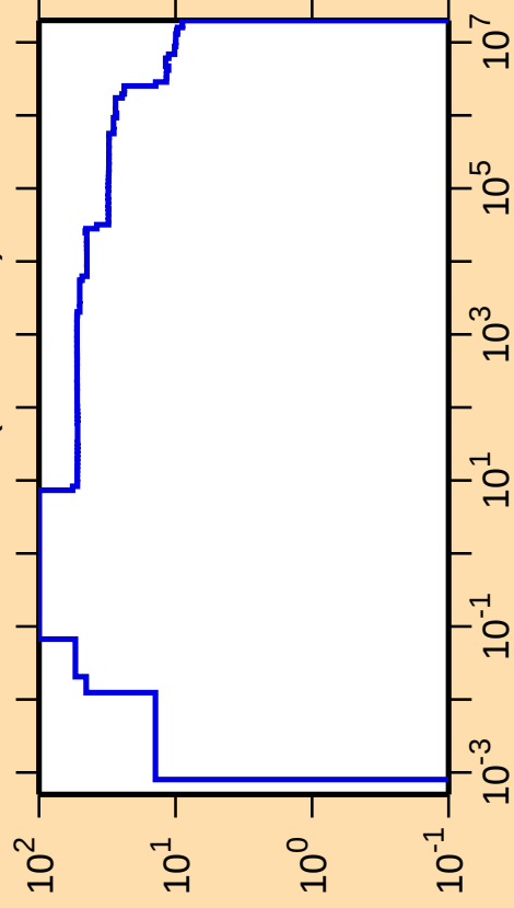
\Delta\sigma/\sigma vs. E for ^{174}\text{Ta}(n,\text{nonel.})
