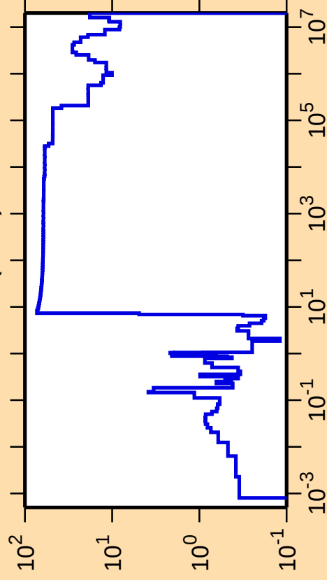
\Delta\sigma/\sigma vs. E for ^{174}\text{Ta}(n,\text{el.})
