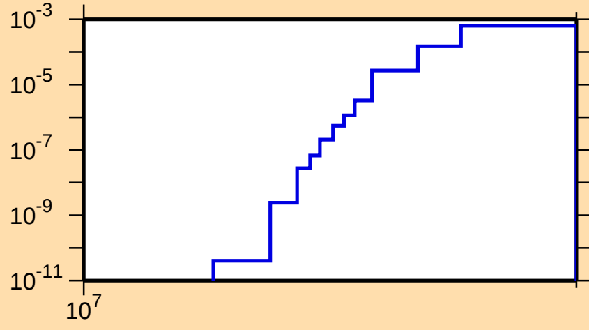
\sigma vs. E for ^{174}\text{Ta}(n,2np)
