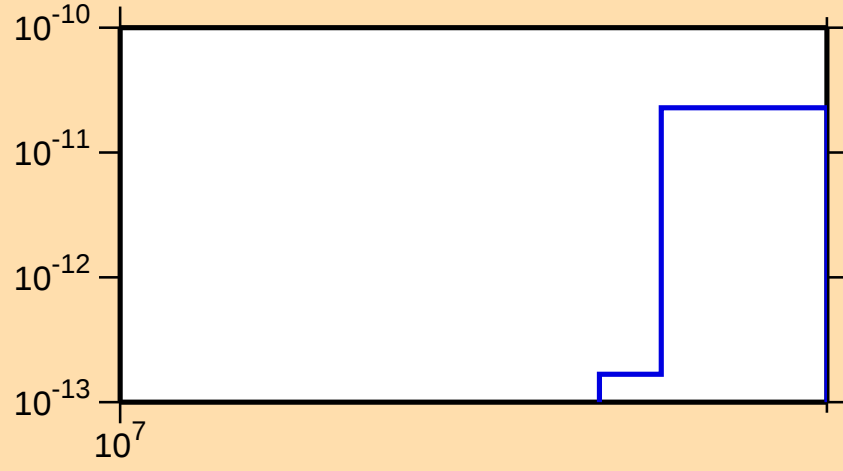
\sigma vs. E for ^{174}\text{Ta}(\text{mt 34})
