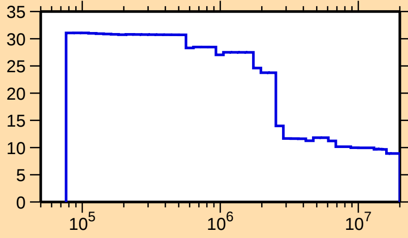
\Delta\sigma/\sigma vs. E for ^{174}\text{Ta}(n,\text{nonel.})
