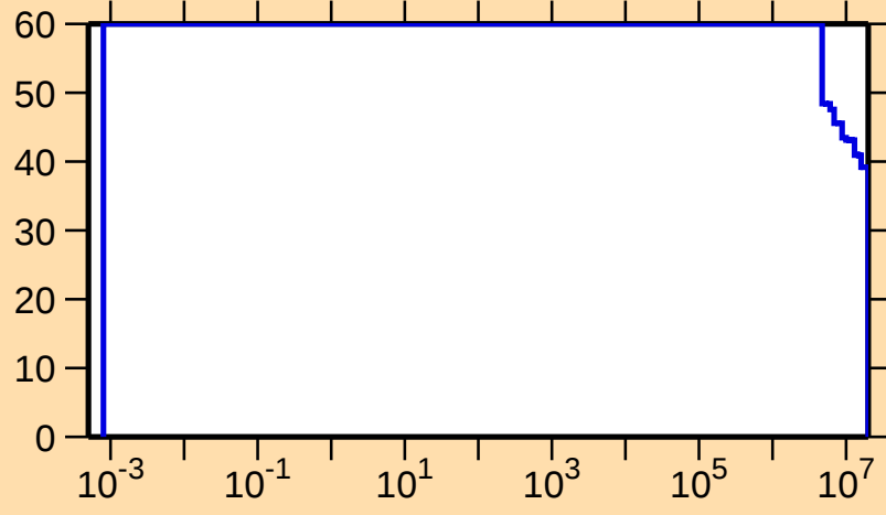
\Delta\sigma/\sigma vs. E for ^{174}\text{Ta}(n,p)
