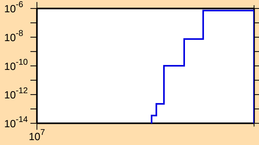
\sigma vs. E for ^{174}\text{Ta}(n,nt)
