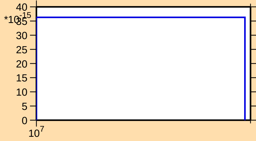
\sigma vs. E for ^{174}\text{Ta}(n,\text{pt})
