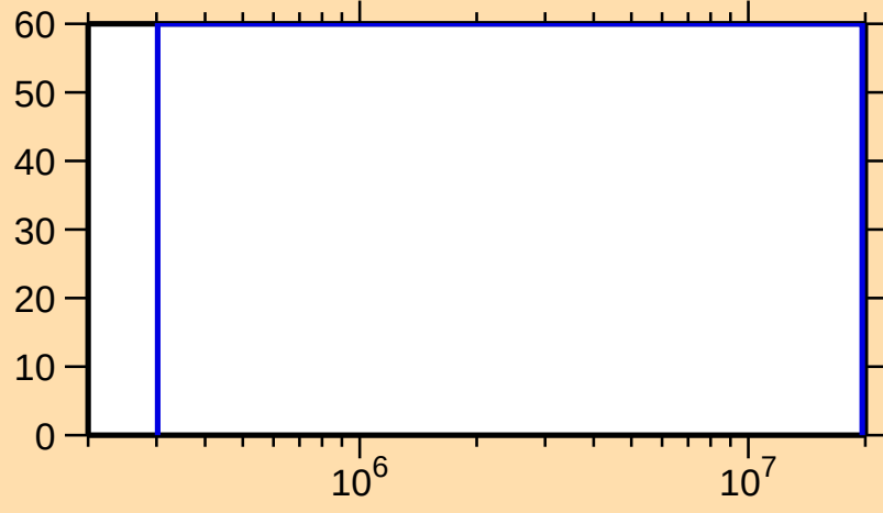
\Delta\sigma/\sigma vs. E for ^{174}\text{Ta}(n,n_1)
