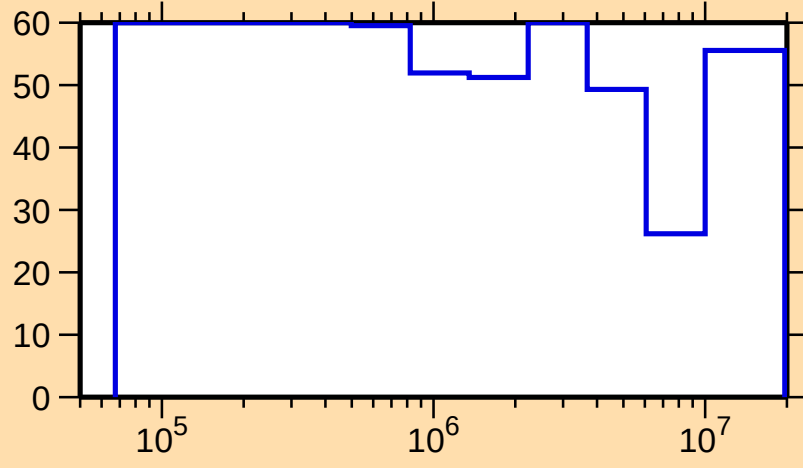
\Delta\sigma/\sigma vs. E for ^{174}\text{Ta}(n,\text{inel.})
