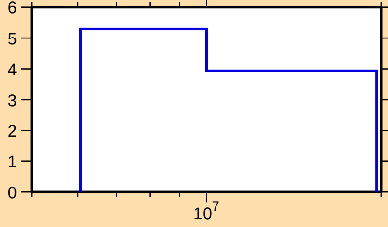
\Delta\sigma/\sigma vs. E for ^{174}\text{Ta}(n,\text{tot.})
