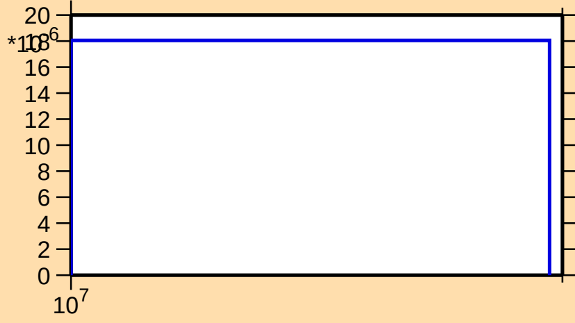
\sigma vs. E for ^{174}\text{Ta}(n,2np)
