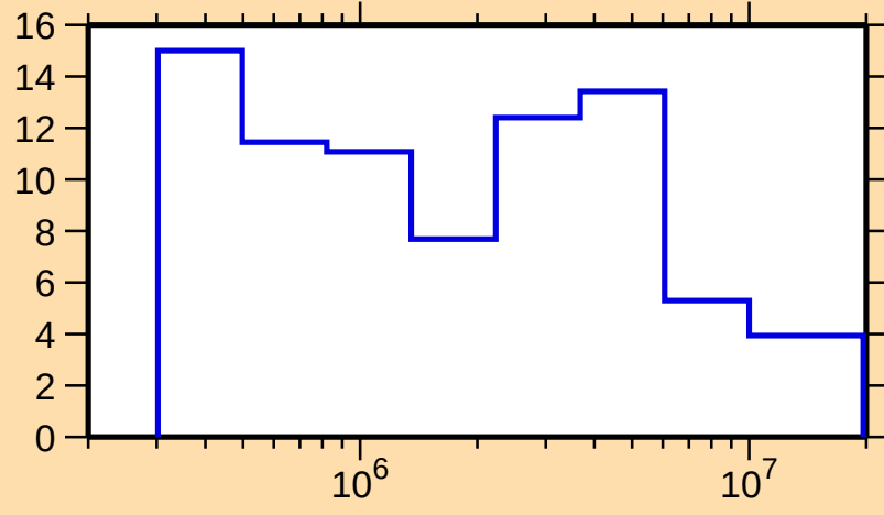
\Delta\sigma/\sigma vs. E for ^{174}\text{Ta}(n,\text{tot.})
