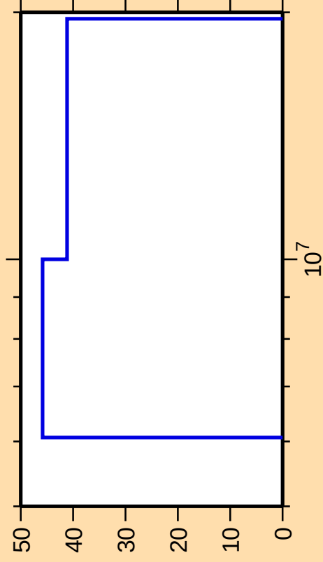
\Delta\sigma/\sigma vs. E for ^{174}\text{Ta}(n,p)
