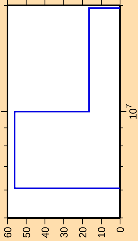
\Delta\sigma/\sigma vs. E for ^{174}\text{Ta}(n,2n)
