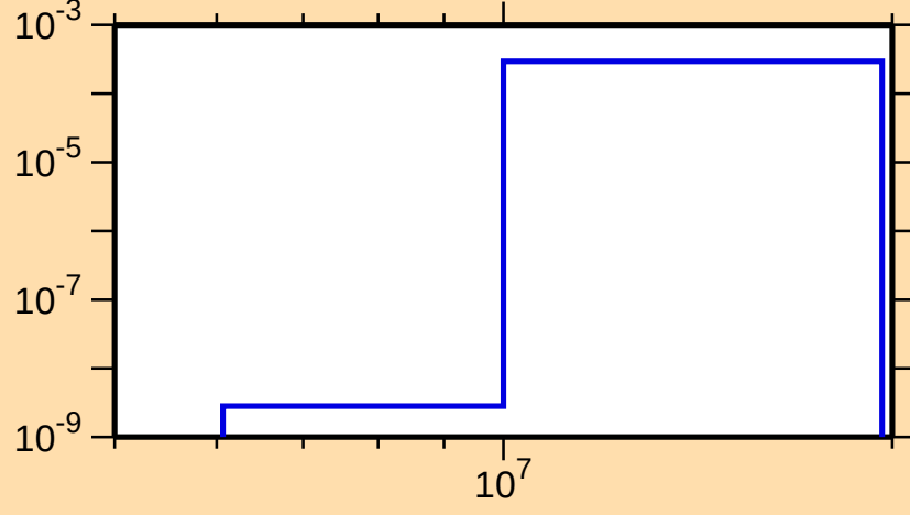
\sigma vs. E for ^{174}\text{Ta}(n,t)
