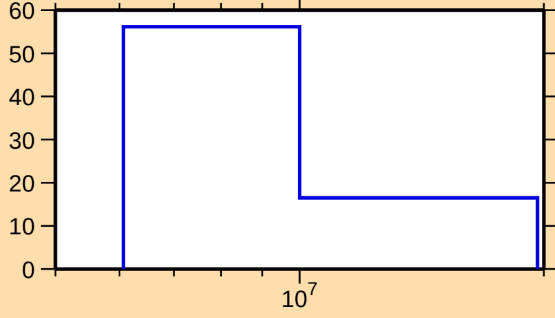
\Delta\sigma/\sigma vs. E for ^{174}\text{Ta}(n,2n)
