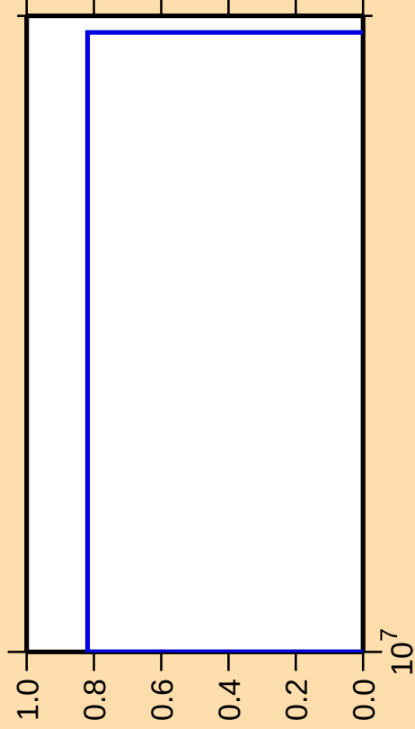
\Delta\sigma/\sigma vs. E for ^{174}\text{Ta}(n,\text{pd})
