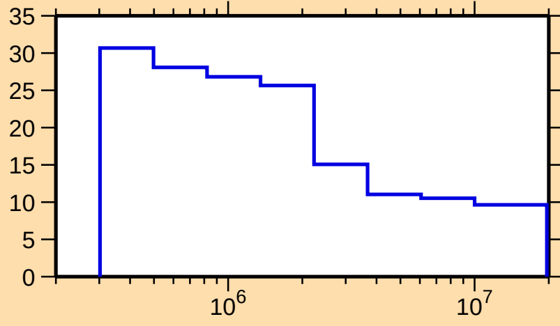
\Delta\sigma/\sigma vs. E for ^{174}\text{Ta}(n,n\text{onel.})
