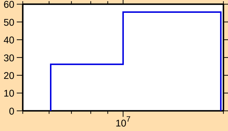
\Delta\sigma/\sigma vs. E for ^{174}\text{Ta}(n,\text{inel.})
