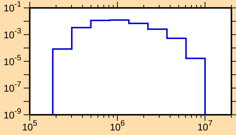
\sigma vs. E for ^{174}\text{Ta}(n,n_3)
