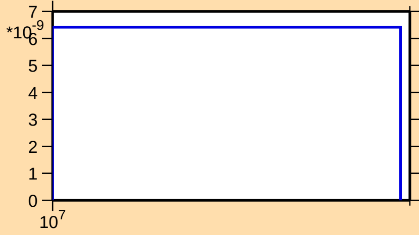
\sigma vs. E for ^{174}\text{Ta}(n,\text{nt})
