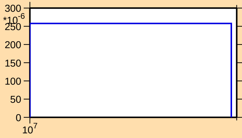
\sigma vs. E for ^{174}\text{Ta}(n,3n)
