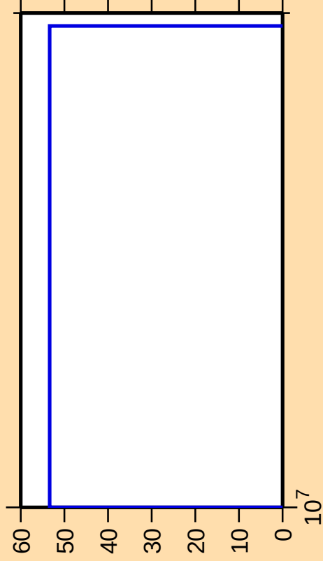
\Delta\sigma/\sigma vs. E for ^{174}\text{Ta}(n,3n)
