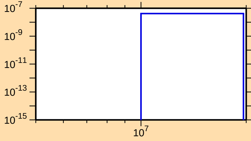
\sigma vs. E for ^{174}\text{Ta}(n,\text{He3})
