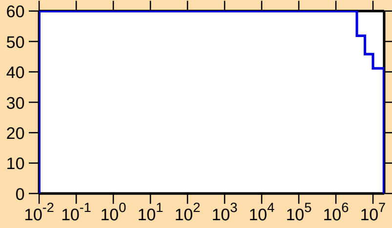
\Delta\sigma/\sigma vs. E for ^{174}\text{Ta}(n,p)
