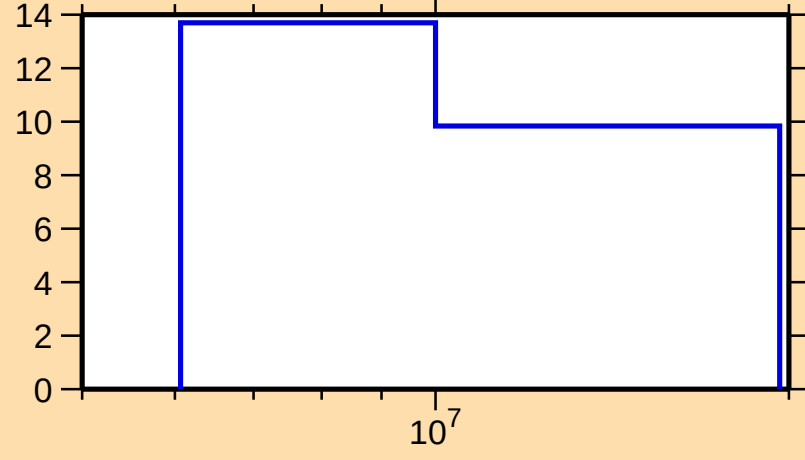
\Delta\sigma/\sigma vs. E for ^{174}\text{Ta}(n,\text{el.})
