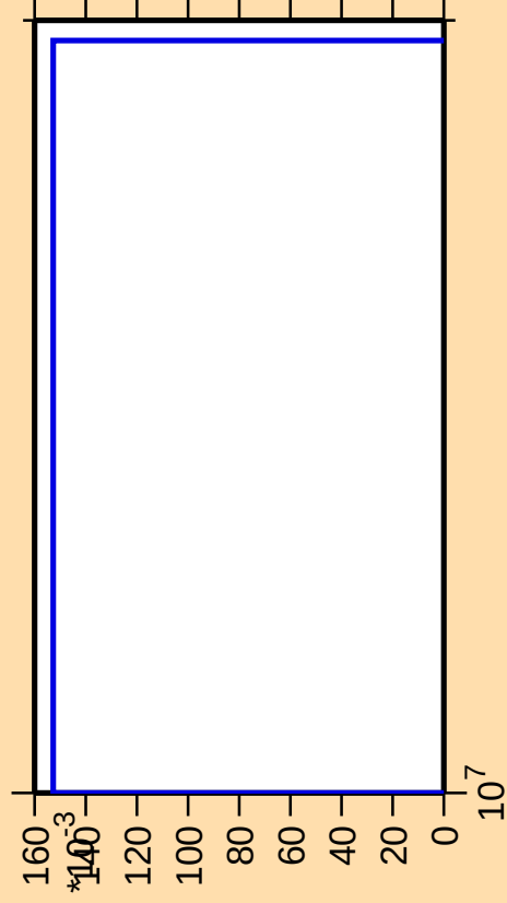
\Delta\sigma/\sigma vs. E for ^{174}\text{Ta}(n,\text{pt})
