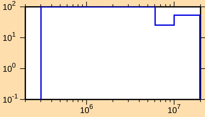
\Delta\sigma/\sigma vs. E for ^{174}\text{Ta}(n,n\text{cont.})
