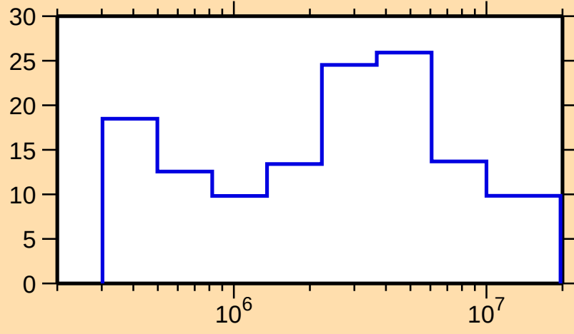
\Delta\sigma/\sigma vs. E for ^{174}\text{Ta}(n,\text{el.})
