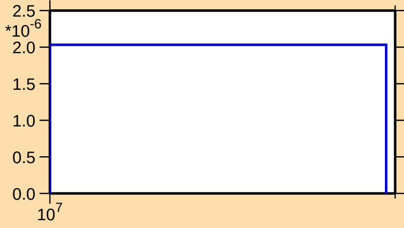
\sigma vs. E for ^{174}\text{Ta}(n,\text{nd})
