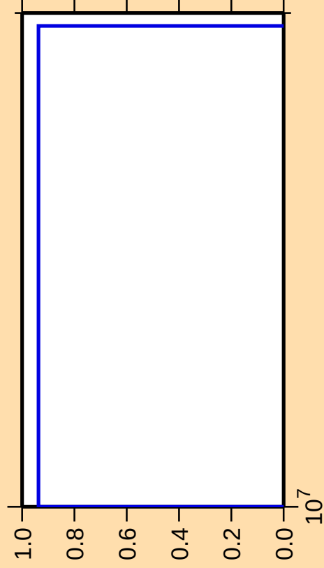
\Delta\sigma/\sigma vs. E for ^{174}\text{Ta}(\text{mt } 34)
