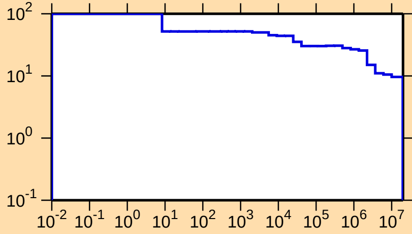
\Delta\sigma/\sigma vs. E for ^{174}\text{Ta}(n,\text{nonel.})
