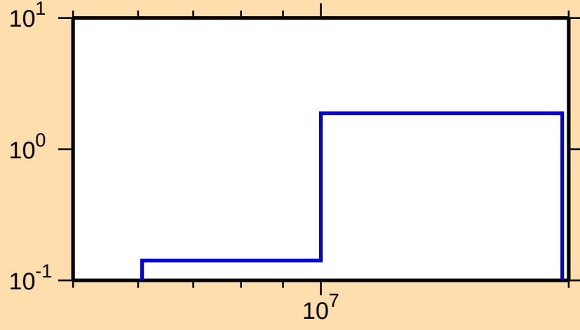
\sigma vs. E for ^{174}\text{Ta}(n,2n)
