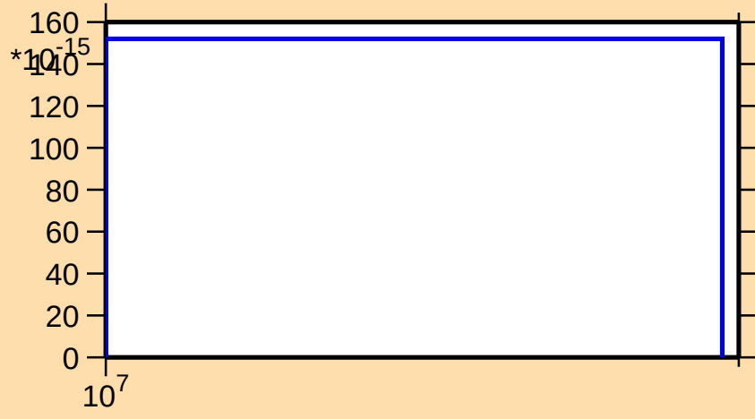
\sigma vs. E for ^{174}\text{Ta}(n,\text{pd})
