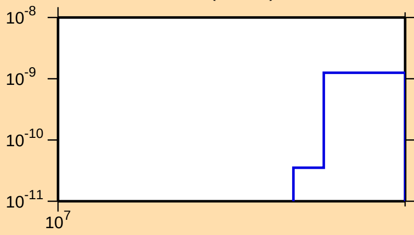
\sigma vs. E for ^{191}\text{Ta}(n,2n\alpha)
