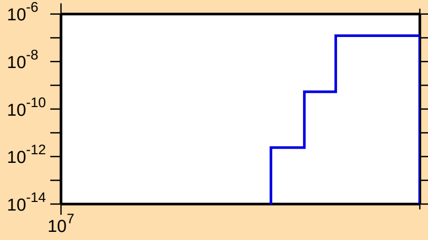
\sigma vs. E for ^{191}\text{Ta}(n,\text{nd})
