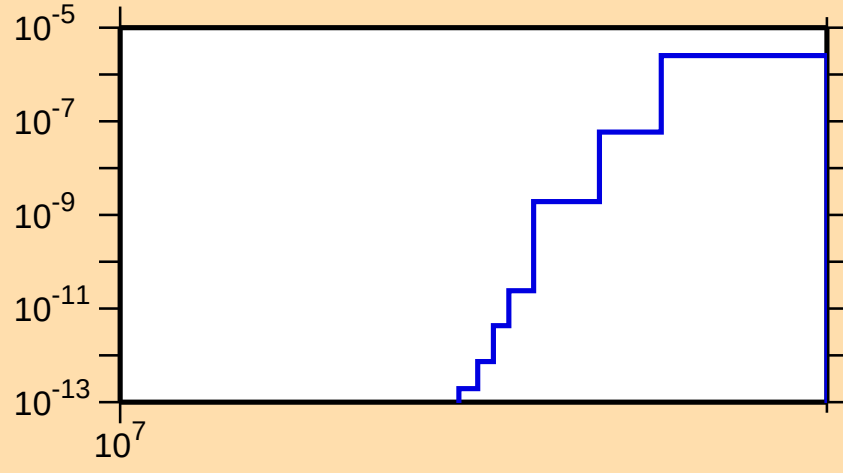
\sigma vs. E for ^{191}\text{Ta}(n,nt)
