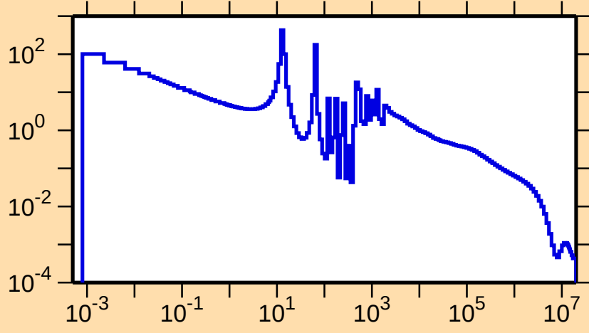
\sigma vs. E for ^{191}\text{Ta}(n,\gamma)
