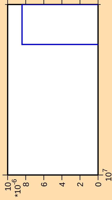
\Delta\sigma/\sigma vs. E for ^{191}\text{Ta}(\text{mt } 42)
