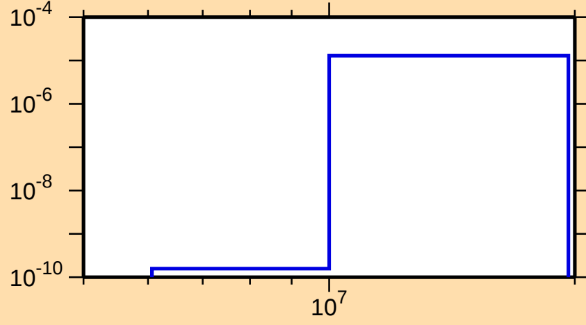
\sigma vs. E for ^{191}\text{Ta}(n,\alpha)
