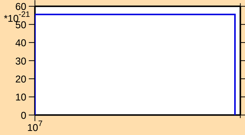
\sigma vs. E for ^{191}\text{Ta}(\text{mt } 42)
