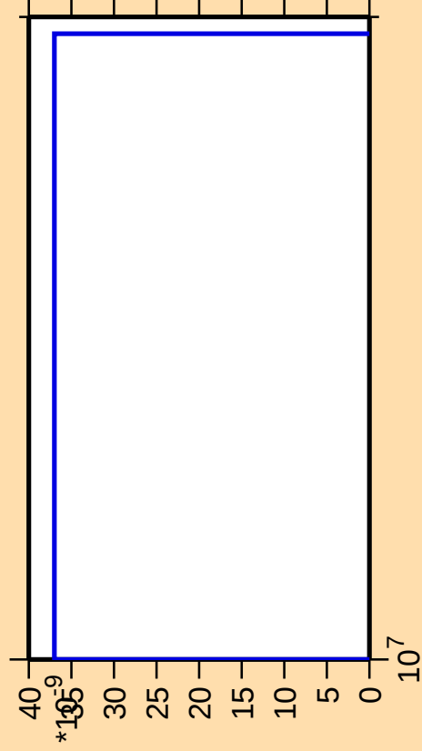
\Delta\sigma/\sigma vs. E for ^{191}\text{Ta}(\text{mt } 42)
