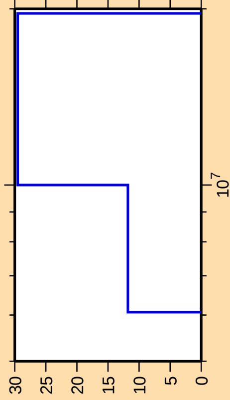
\Delta\sigma/\sigma vs. E for ^{191}\text{Ta}(n,2n)
