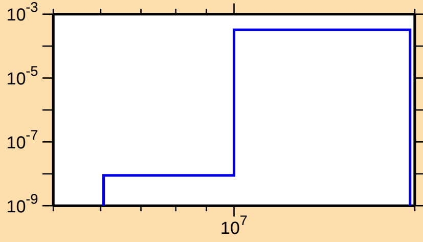
\sigma vs. E for ^{191}\text{Ta}(n,p)
