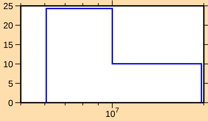
\Delta\sigma/\sigma vs. E for ^{191}\text{Ta}(n,\text{el.})
