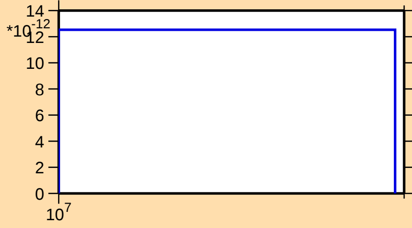
\sigma vs. E for ^{191}\text{Ta}(n,2n\alpha)
