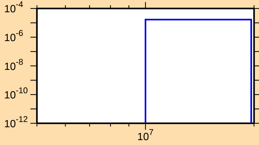
\sigma vs. E for ^{191}\text{Ta}(n,np)
