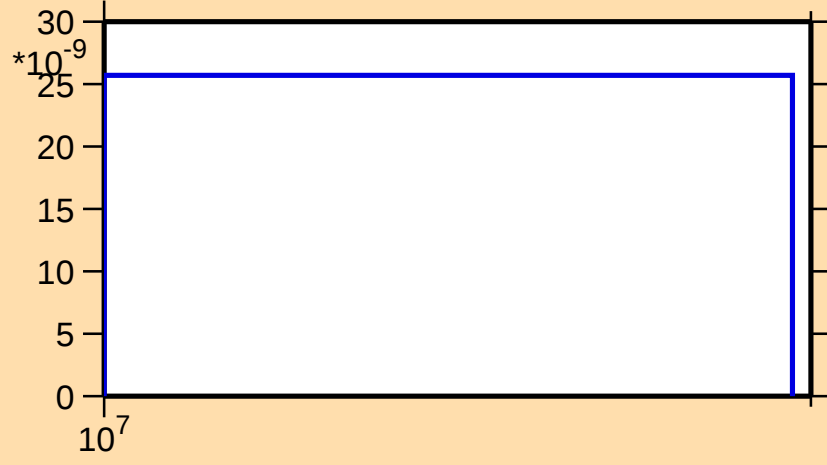
\sigma vs. E for ^{191}\text{Ta}(n,\text{nt})
