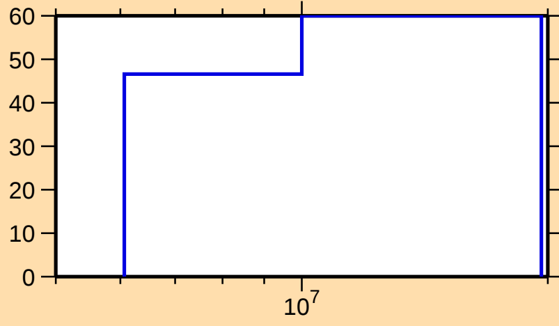
\Delta\sigma/\sigma vs. E for ^{191}\text{Ta}(n,n\text{cont.})
