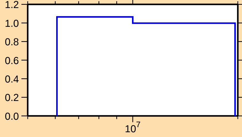
\sigma vs. E for ^{191}\text{Ta}(n,2n)
