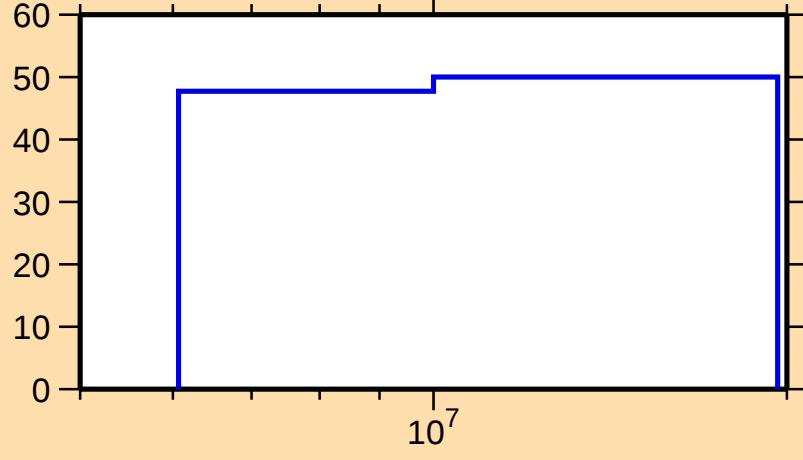
\Delta\sigma/\sigma vs. E for ^{191}\text{Ta}(n,p)
