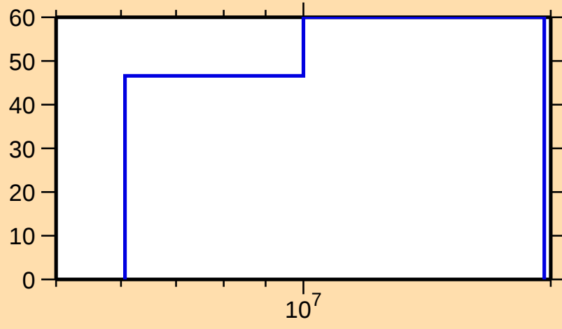
\Delta\sigma/\sigma vs. E for ^{191}\text{Ta}(n,\text{ncont.})
