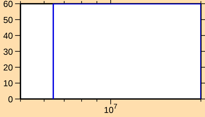
\Delta\sigma/\sigma vs. E for ^{191}\text{Ta}(n,n_1)
