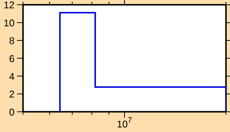
\Delta\sigma/\sigma vs. E for ^{191}\text{Ta}(n,\text{tot.})
