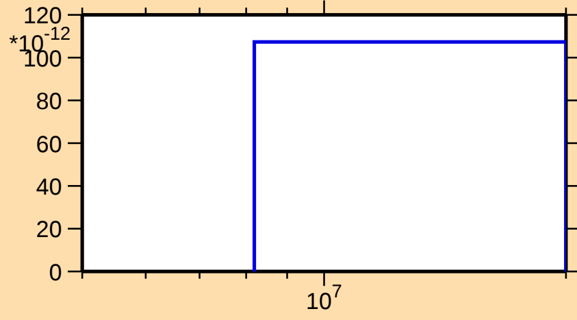
\sigma vs. E for ^{191}\text{Ta}(n,2np)
