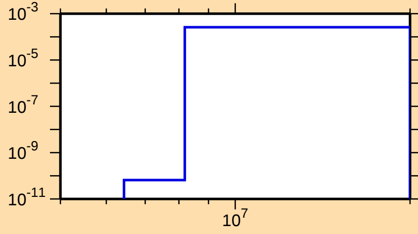
\sigma vs. E for ^{191}\text{Ta}(n,p)
