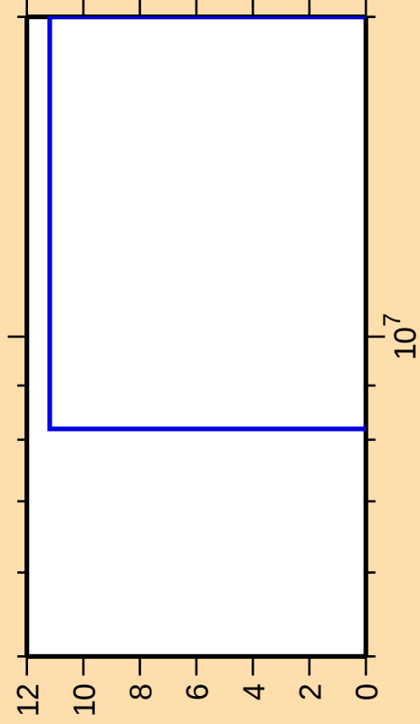
\Delta\sigma/\sigma vs. E for ^{191}\text{Ta}(n,3n)
