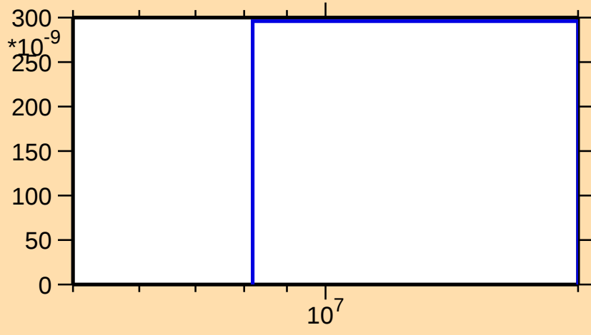
\sigma vs. E for ^{191}\text{Ta}(n,n\alpha)
