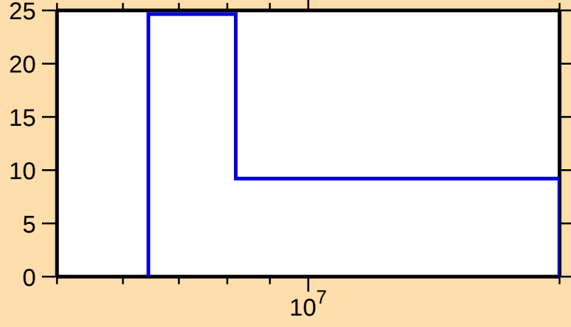
\Delta\sigma/\sigma vs. E for ^{191}\text{Ta}(n,\text{el.})
