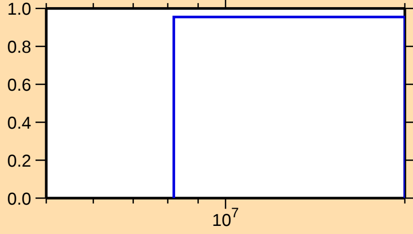
\sigma vs. E for ^{191}\text{Ta}(n,3n)
