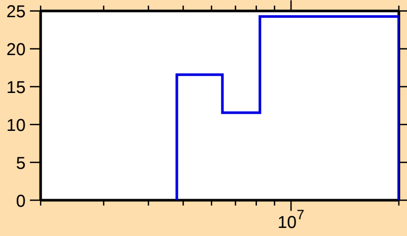
\Delta\sigma/\sigma vs. E for ^{191}\text{Ta}(n,2n)
