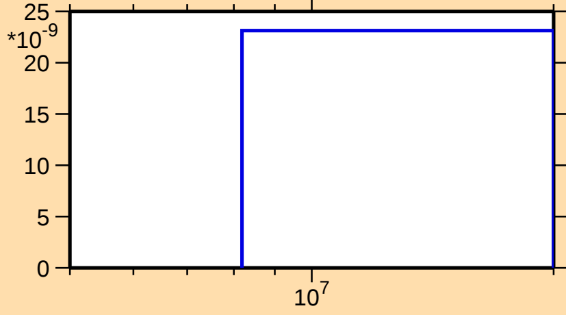
\sigma vs. E for ^{191}\text{Ta}(n,nt)
