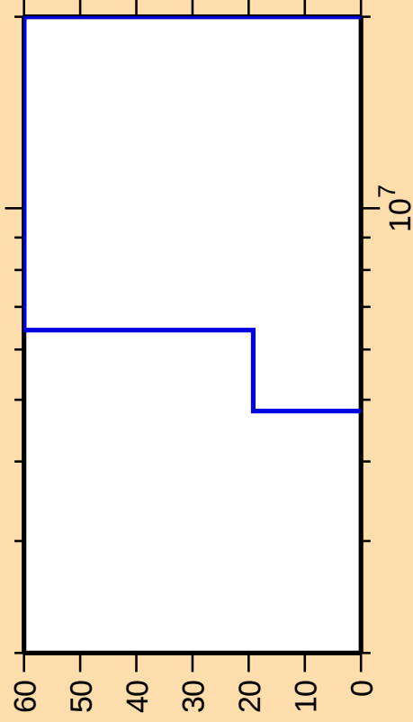
\Delta\sigma/\sigma vs. E for ^{191}\text{Ta}(n,n\text{cont.})
