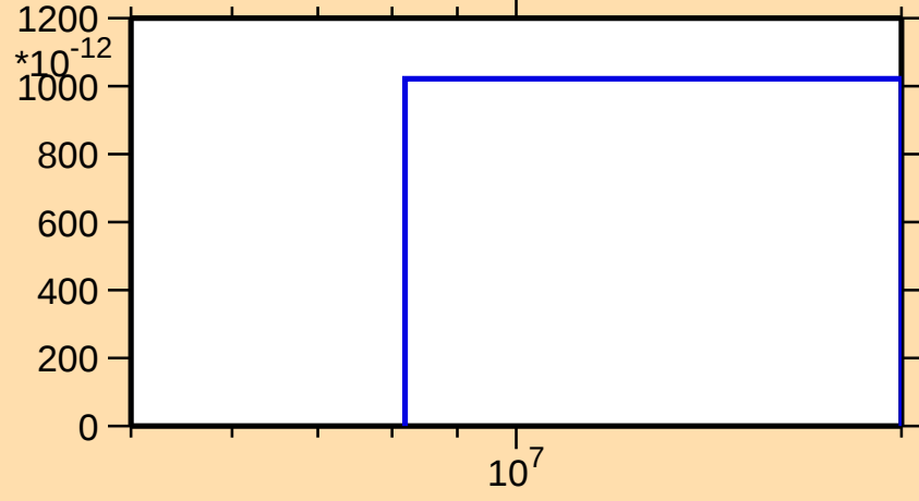
\sigma vs. E for ^{191}\text{Ta}(n,\text{nd})
