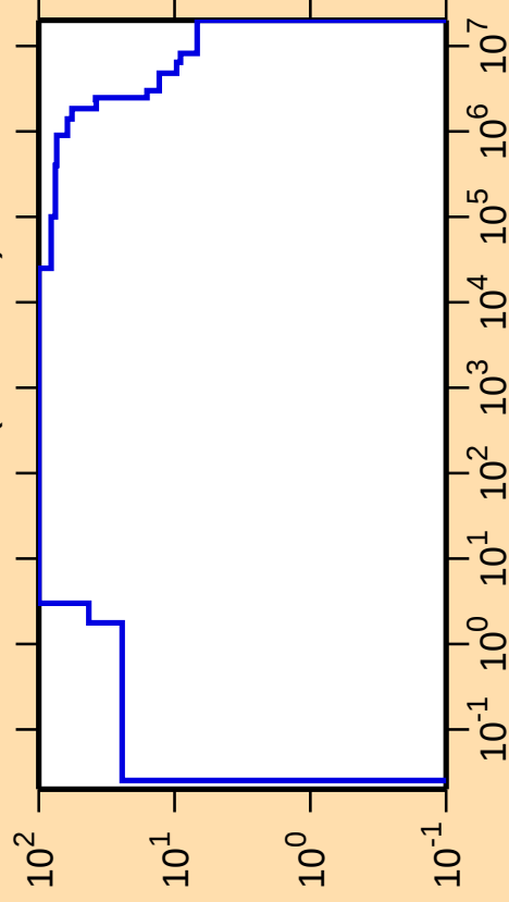
\Delta\sigma/\sigma vs. E for ^{191}\text{Ta}(n,\text{nonel.})
