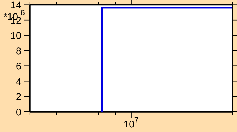
\sigma vs. E for ^{191}\text{Ta}(n,np)
