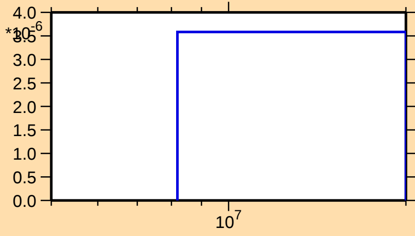
\sigma vs. E for ^{191}\text{Ta}(n,t)
