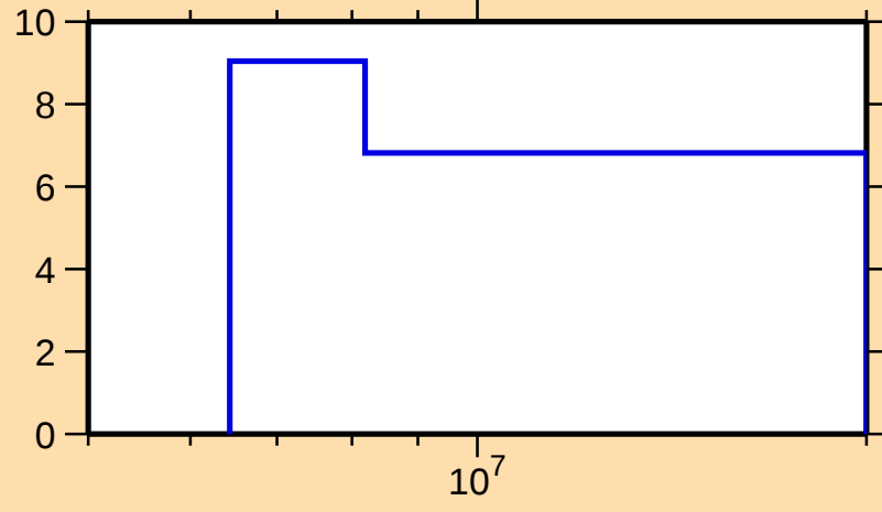
\Delta\sigma/\sigma vs. E for ^{191}\text{Ta}(n,\text{nonel.})
