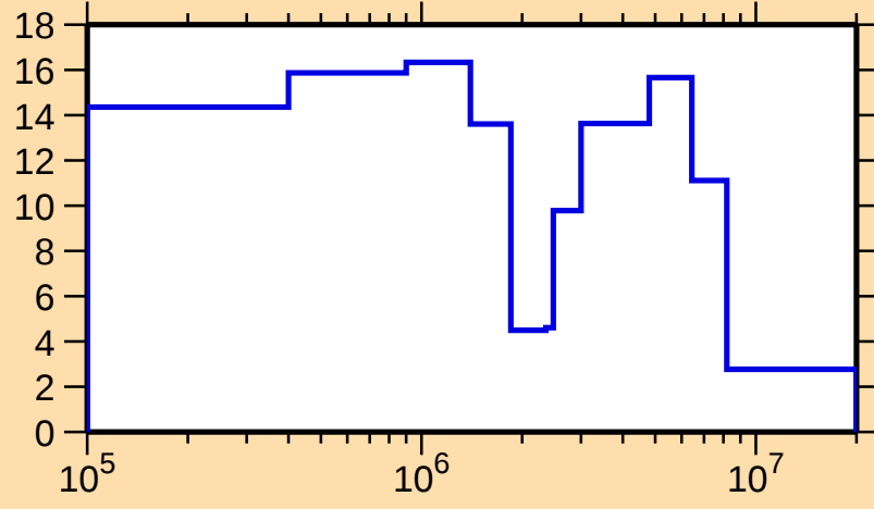
\Delta\sigma/\sigma vs. E for ^{191}\text{Ta}(n,\text{tot.})
