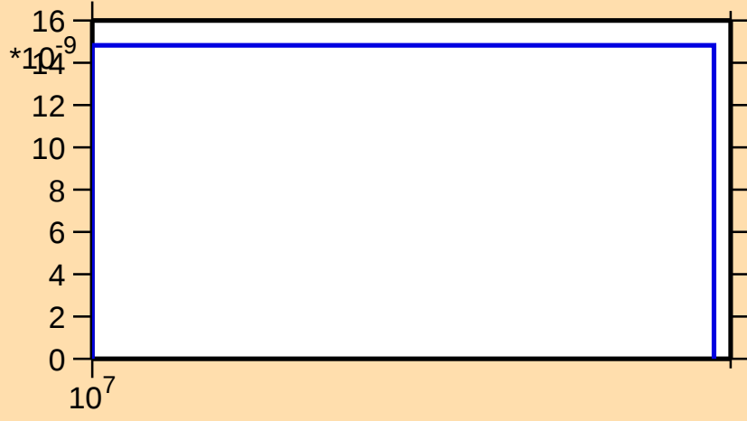
\sigma vs. E for ^{139}\text{Tb}(n,\text{nd})
