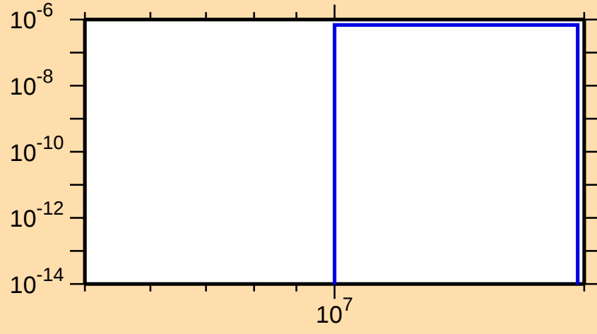
\sigma vs. E for ^{139}\text{Tb}(n,\text{pt})
