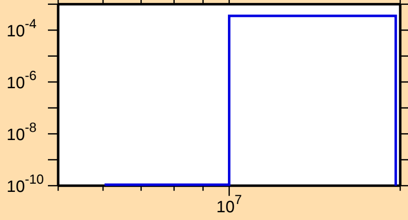
\sigma vs. E for ^{139}\text{Tb}(n,t)
