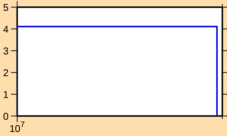
\Delta\sigma/\sigma vs. E for ^{139}\text{Tb}(n,\text{tot.})
