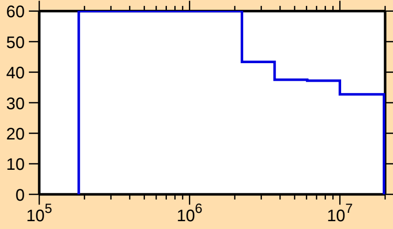
\Delta\sigma/\sigma vs. E for ^{139}\text{Tb}(n,n\text{cont.})
