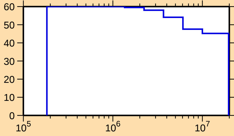
\Delta\sigma/\sigma vs. E for ^{139}\text{Tb}(n,\text{inel.})
