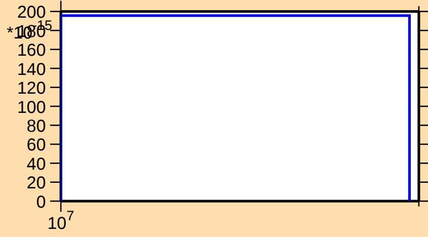
\sigma vs. E for ^{139}\text{Tb}(n,\text{nt})
