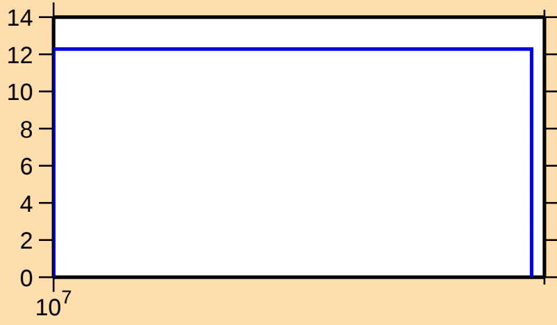
\Delta\sigma/\sigma vs. E for ^{139}\text{Tb}(n,\text{el.})
