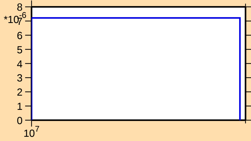
\sigma vs. E for ^{139}\text{Tb}(n,2np)
