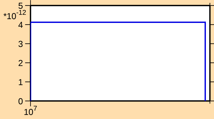
\sigma vs. E for ^{139}\text{Tb}(n,2n\alpha)
