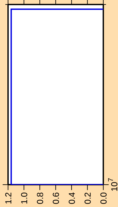
\Delta\sigma/\sigma vs. E for ^{139}\text{Tb}(n,\text{nt})
