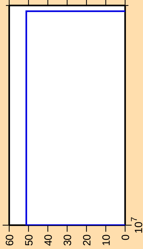
\Delta\sigma/\sigma vs. E for ^{139}\text{Tb}(\text{mt } 34)
