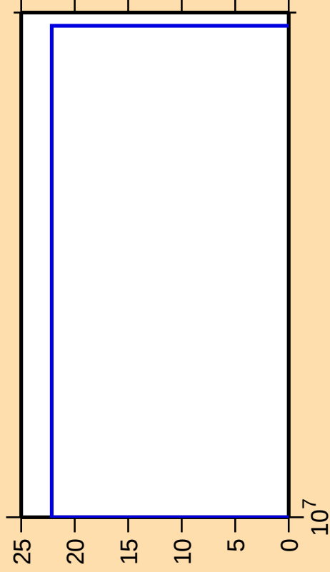
\Delta\sigma/\sigma vs. E for ^{139}\text{Tb}(n,2n\alpha)
