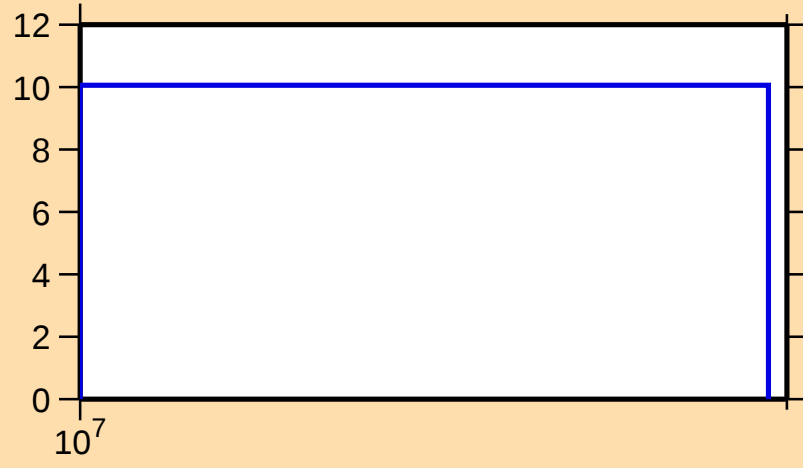
\Delta\sigma/\sigma vs. E for ^{139}\text{Tb}(n,\text{nonel.})
