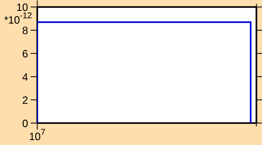
\sigma vs. E for ^{139}\text{Tb}(\text{mt } 34)
