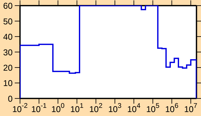
\Delta\sigma/\sigma vs. E for ^{141}\text{Tb}(n,\text{tot.})
