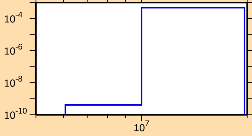
\sigma vs. E for ^{141}\text{Tb}(n,t)
