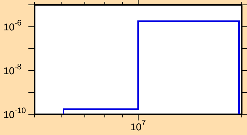
\sigma vs. E for ^{141}\text{Tb}(\text{mt117})
