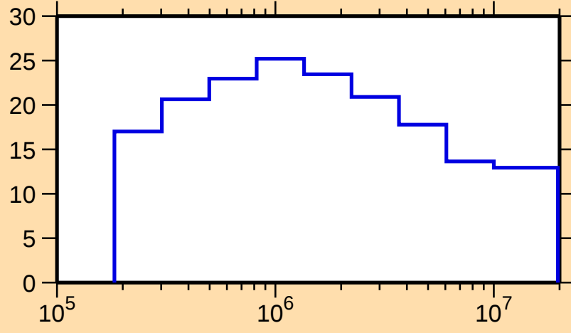
\Delta\sigma/\sigma vs. E for ^{141}\text{Tb}(n,n\text{onel.})
