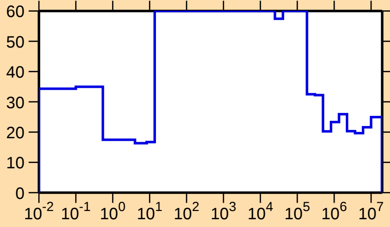
\Delta\sigma/\sigma vs. E for ^{141}\text{Tb}(n,\text{tot.})
