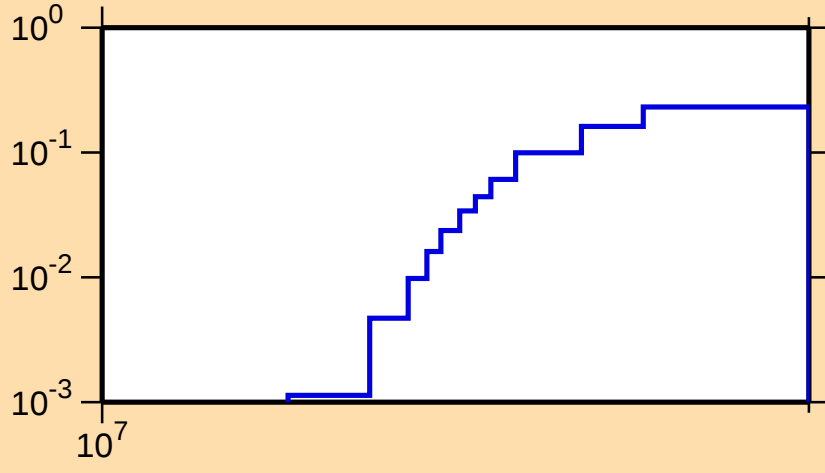
\sigma vs. E for ^{145}\text{Tb}(n,2n)
