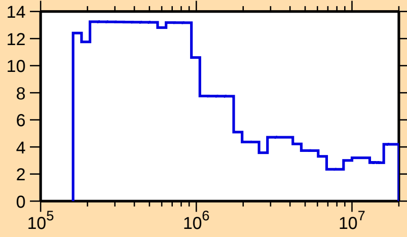
\Delta\sigma/\sigma vs. E for ^{145}\text{Tb}(n,\text{nonel.})
