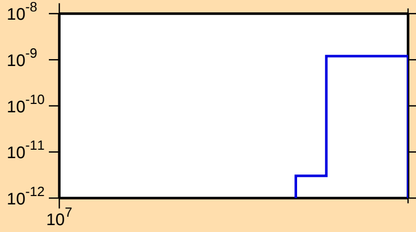
\sigma vs. E for ^{145}\text{Tb}(n,2n\alpha)
