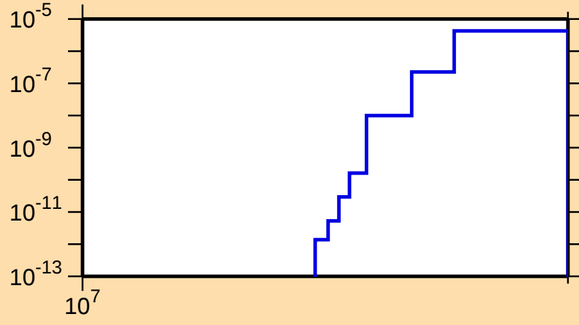
\sigma vs. E for ^{145}\text{Tb}(n,\text{nd})
