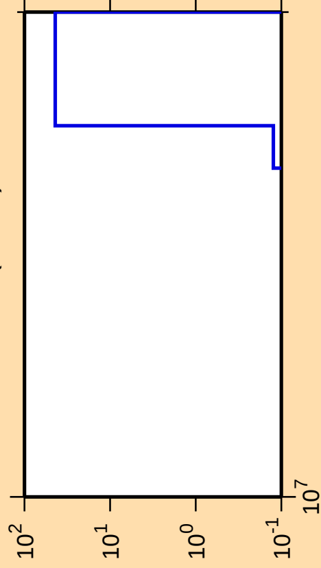
\Delta\sigma/\sigma vs. E for ^{145}\text{Tb}(\text{mt } 34)
