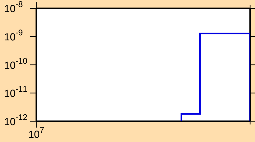
\sigma vs. E for ^{145}\text{Tb}(n,\text{pt})
