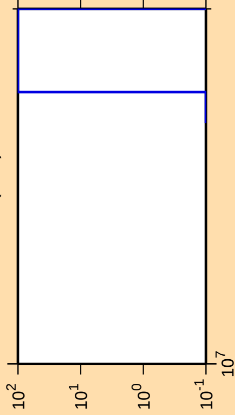
\Delta\sigma/\sigma vs. E for ^{145}\text{Tb}(n,\text{nt})
