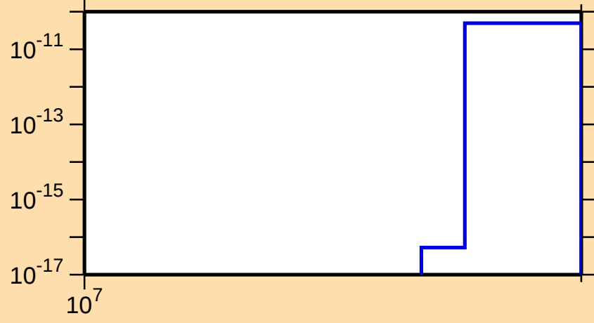
\sigma vs. E for ^{145}\text{Tb}(n,\text{nt})
