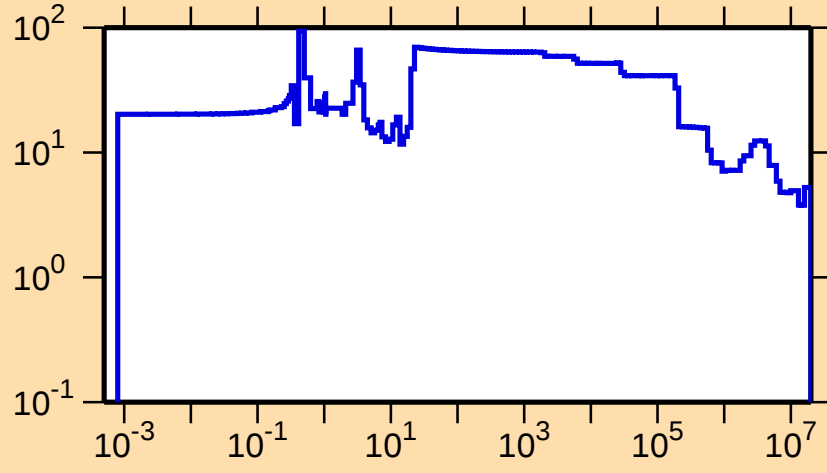
\Delta\sigma/\sigma vs. E for ^{145}\text{Tb}(n,\text{el.})
