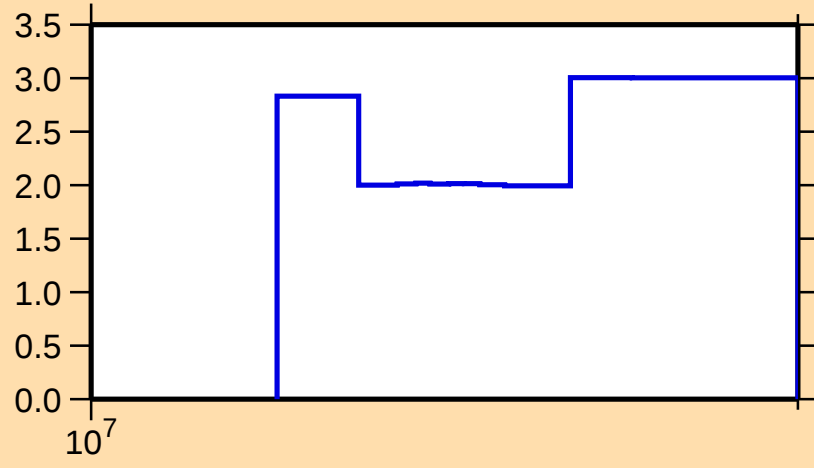
\Delta\sigma/\sigma vs. E for ^{145}\text{Tb}(n,\text{tot.})
