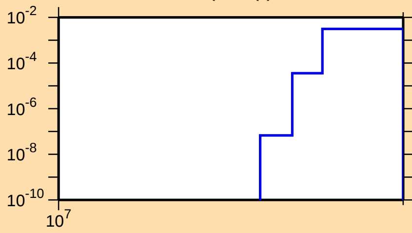
\sigma vs. E for ^{145}\text{Tb}(n,2np)
