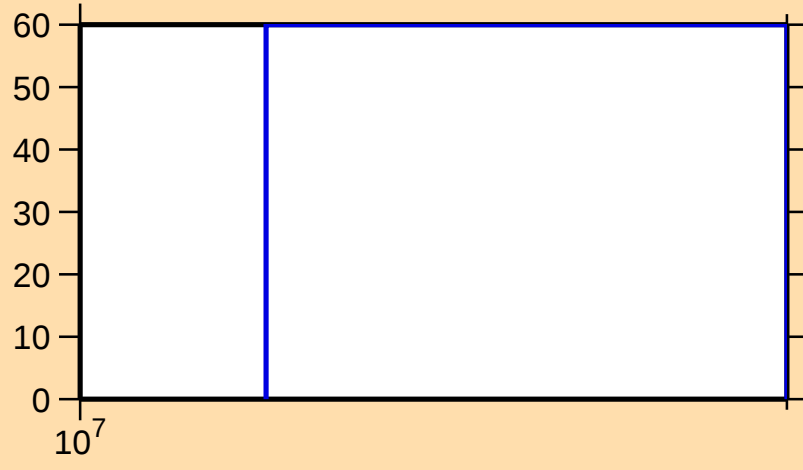
\Delta\sigma/\sigma vs. E for ^{145}\text{Tb}(n,\text{inel.})
