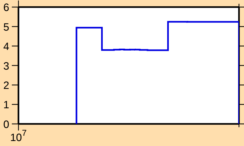
\Delta\sigma/\sigma vs. E for ^{145}\text{Tb}(n,\text{el.})
