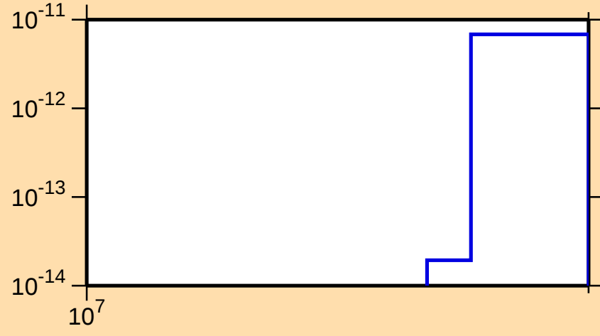
\sigma vs. E for ^{145}\text{Tb}(\text{mt } 34)
