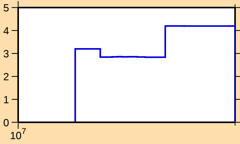
\Delta\sigma/\sigma vs. E for ^{145}\text{Tb}(n,\text{nonel.})
