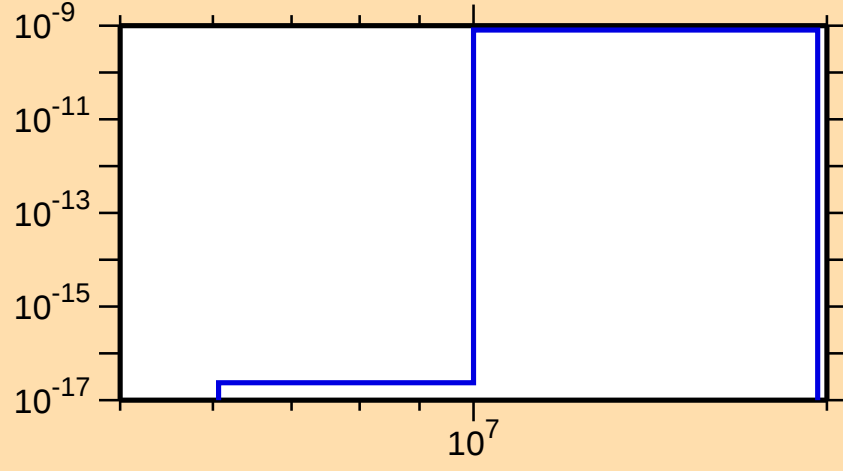
\sigma vs. E for ^{145}\text{Tb}(\text{mt117})
