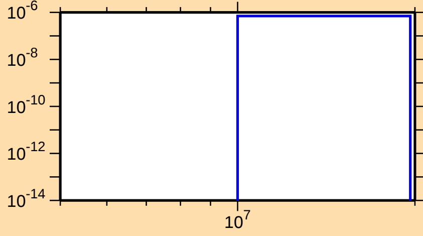
\sigma vs. E for ^{145}\text{Tb}(\text{mt } 45)
