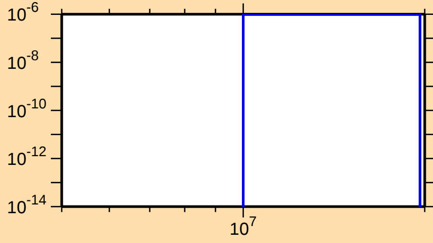
\sigma vs. E for ^{145}\text{Tb}(n,\text{pd})
