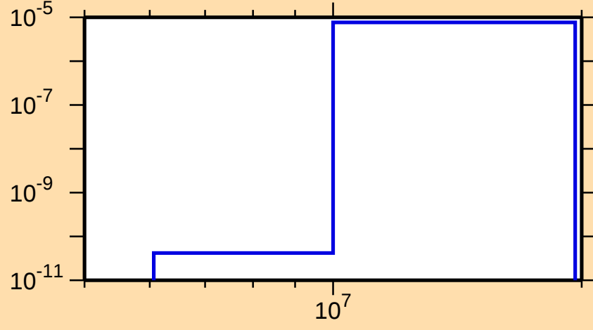
\sigma vs. E for ^{145}\text{Tb}(n,\text{He3})
