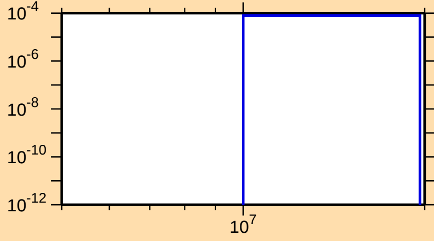
\sigma vs. E for ^{145}\text{Tb}(n,t)
