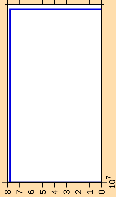
\Delta\sigma/\sigma vs. E for ^{145}\text{Tb}(n,2n\alpha)
