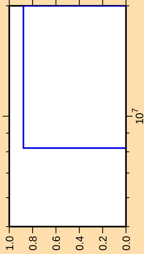
\Delta\sigma/\sigma vs. E for ^{145}\text{Tb}(n,nt)
