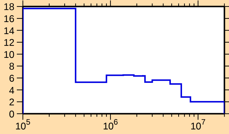
\Delta\sigma/\sigma vs. E for ^{145}\text{Tb}(n,\text{tot.})
