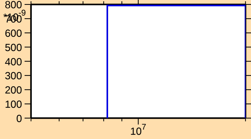
\sigma vs. E for ^{145}\text{Tb}(n,\text{pd})
