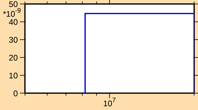
\sigma vs. E for ^{145}\text{Tb}(n,\text{nd})
