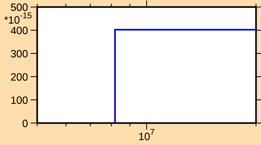
\sigma vs. E for ^{145}\text{Tb}(n,nt)
