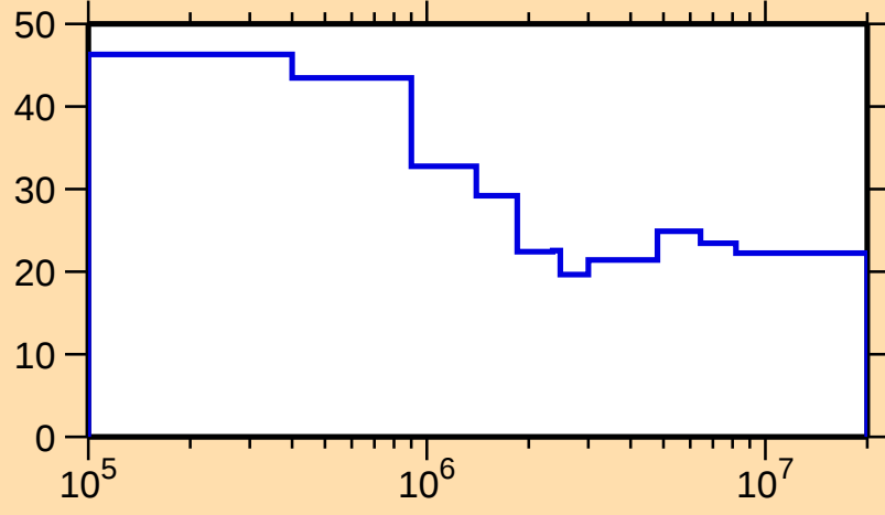
\Delta\sigma/\sigma vs. E for ^{145}\text{Tb}(n,n_1)
