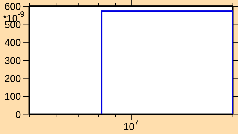
\sigma vs. E for ^{145}\text{Tb}(\text{mt } 45)
