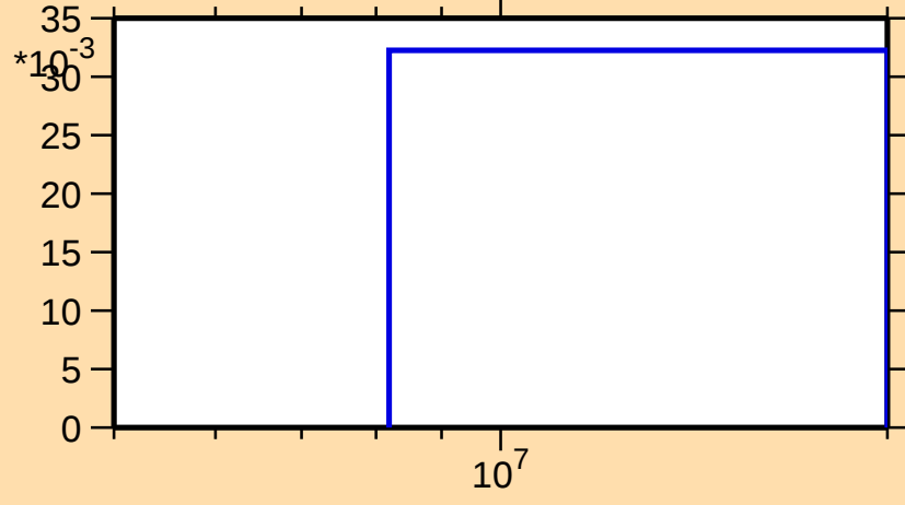
\sigma vs. E for ^{145}\text{Tb}(n,2n)
