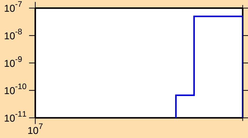
\sigma vs. E for ^{148}\text{Tb}(n,\text{nt})
