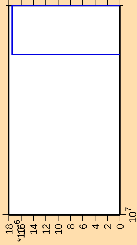
\Delta\sigma/\sigma vs. E for ^{148}\text{Tb}(\text{mt } 11)
