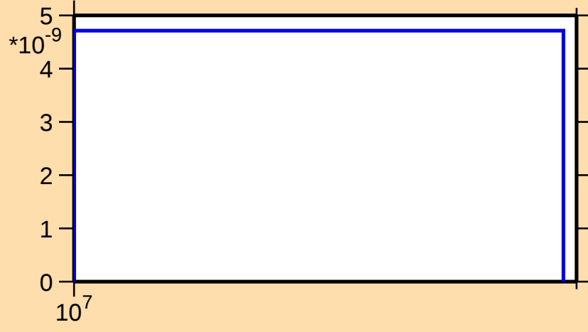
\sigma vs. E for ^{148}\text{Tb}(n,\text{pt})
