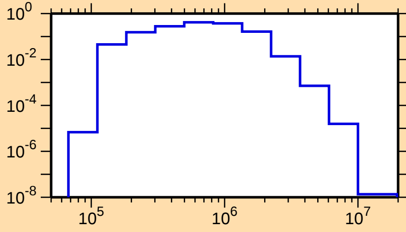
\sigma vs. E for ^{148}\text{Tb}(n,n_2)
