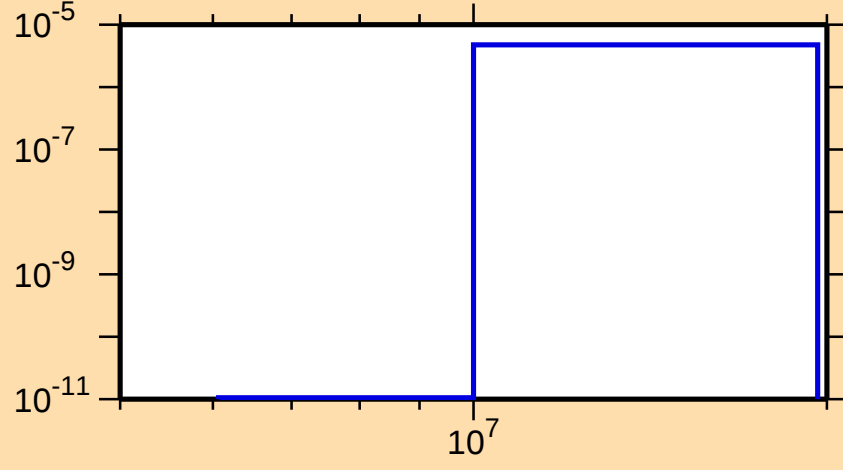
\sigma vs. E for ^{148}\text{Tb}(n,\text{He3})
