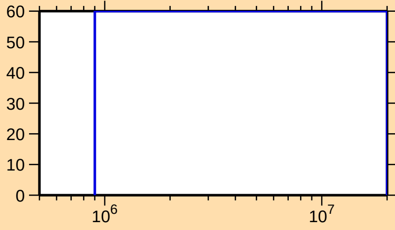
\Delta\sigma/\sigma vs. E for ^{148}\text{Tb}(n,n_1)
