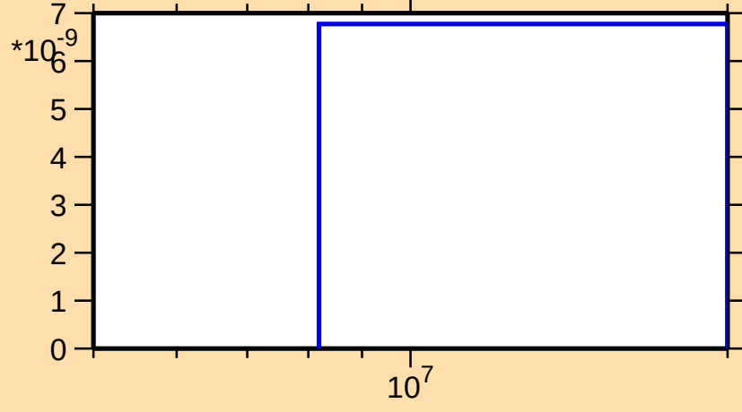
\sigma vs. E for ^{148}\text{Tb}(n,\text{pd})
