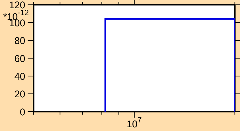
\sigma vs. E for ^{148}\text{Tb}(\text{mt } 34)
