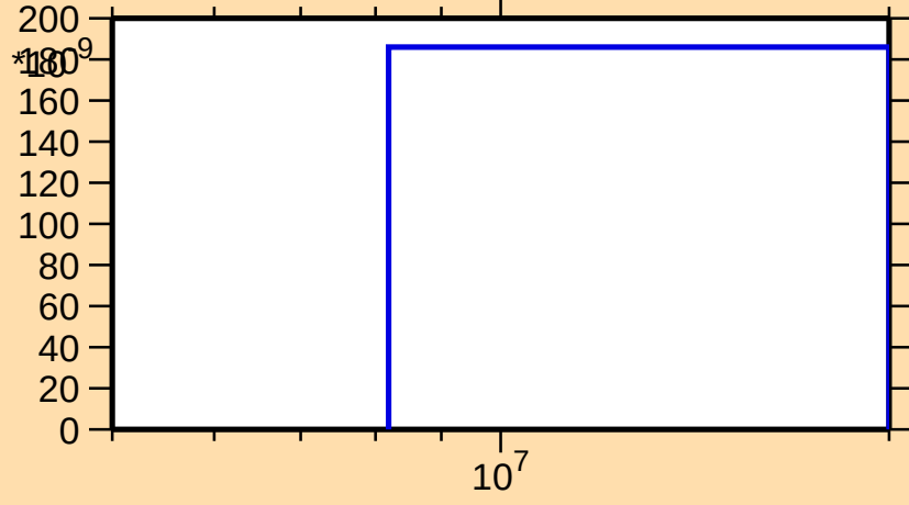
\sigma vs. E for ^{148}\text{Tb}(n,3n)
