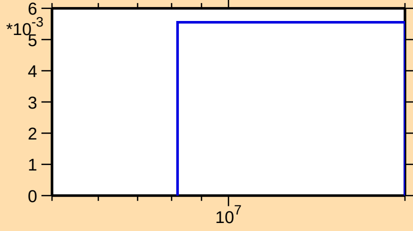
\sigma vs. E for ^{148}\text{Tb}(n,2np)
