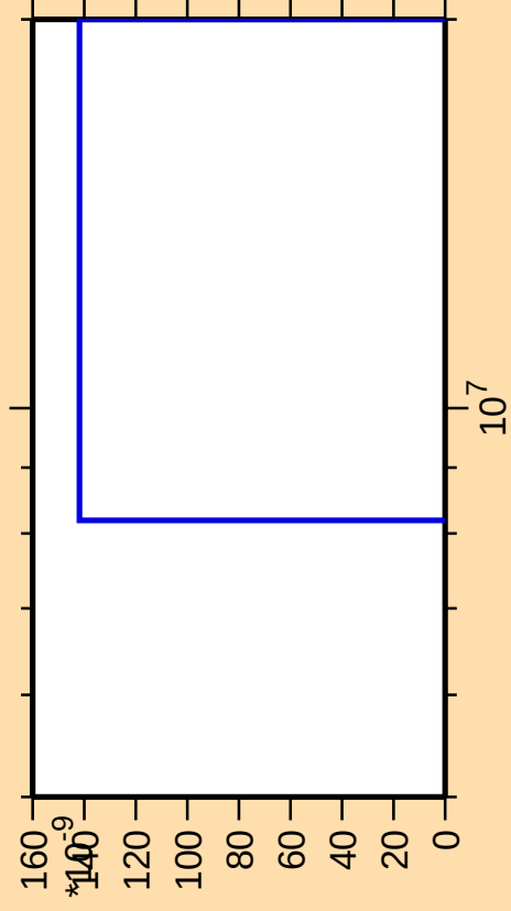
\Delta\sigma/\sigma vs. E for ^{148}\text{Tb}(\text{mt } 11)
