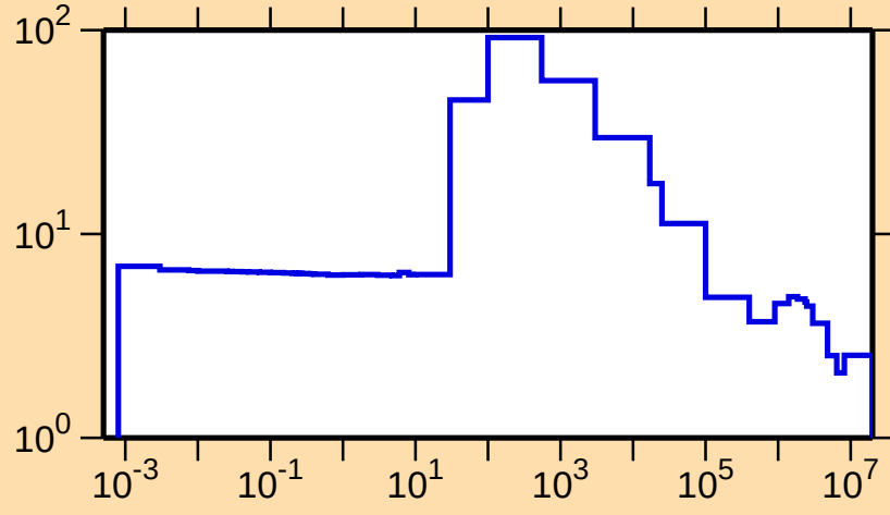
\sigma vs. E for ^{148}\text{Tb}(n,\text{el.})
