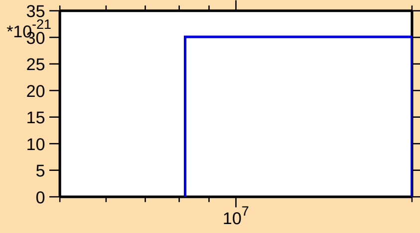
\sigma vs. E for ^{148}\text{Tb}(\text{mt } 11)
