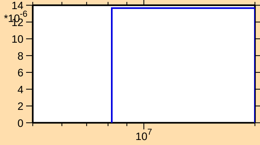
\sigma vs. E for ^{151}\text{Tb}(n,2np)
