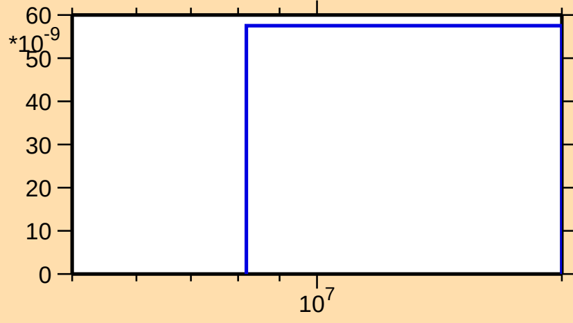
\sigma vs. E for ^{151}\text{Tb}(n,\text{He3})
