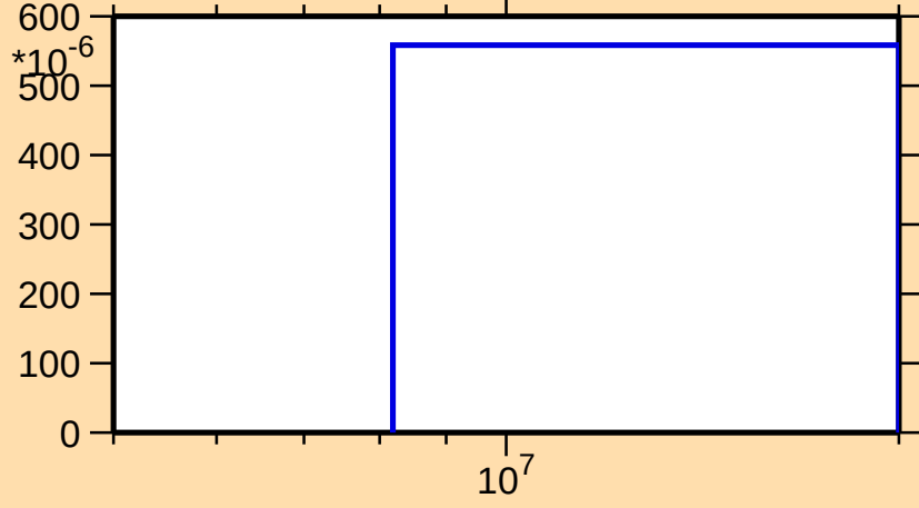
\sigma vs. E for ^{151}\text{Tb}(n,3n)
