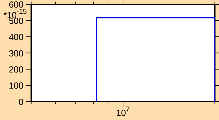
\sigma vs. E for ^{151}\text{Tb}(n,3n\alpha)
