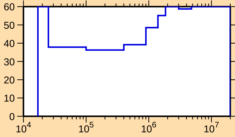
\Delta\sigma/\sigma vs. E for ^{151}\text{Tb}(n,n_1)
