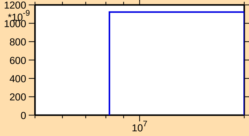
\sigma vs. E for ^{151}\text{Tb}(n,\text{nd})
