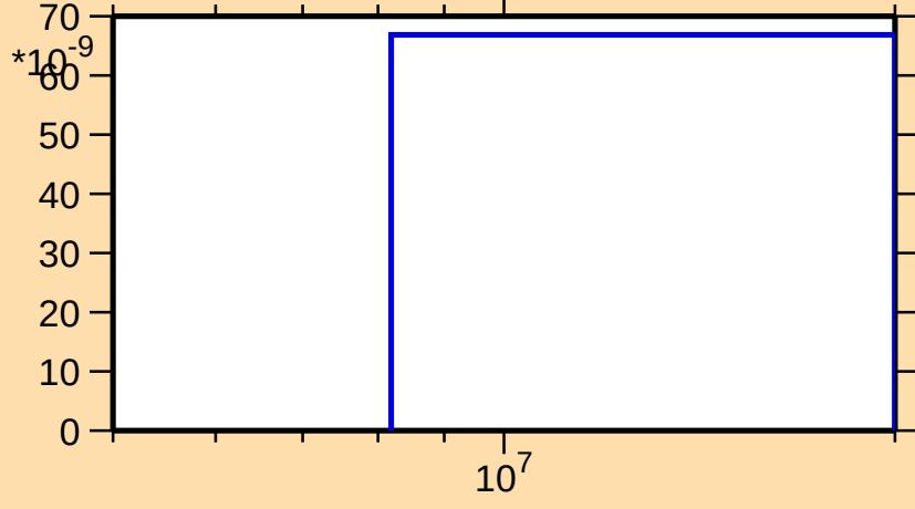
\sigma vs. E for ^{151}\text{Tb}(n,nt)
