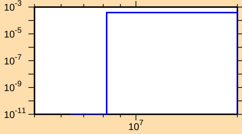
\sigma vs. E for ^{151}\text{Tb}(n,t)
