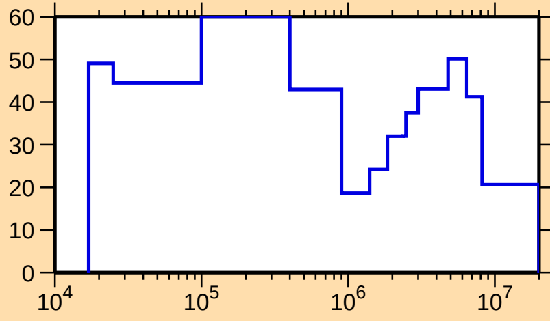
\Delta\sigma/\sigma vs. E for ^{151}\text{Tb}(n,\text{el.})
