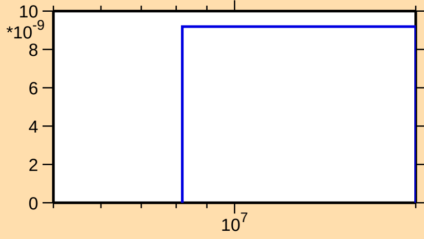
\sigma vs. E for ^{151}\text{Tb}(\text{mt } 45)
