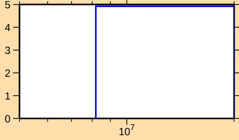
\Delta\sigma/\sigma vs. E for ^{151}\text{Tb}(n,\text{nonel.})
