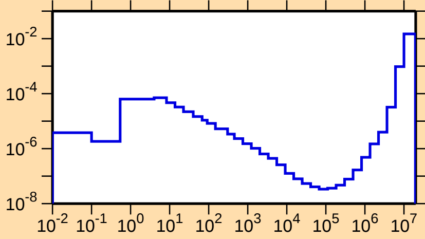
\sigma vs. E for ^{158}\text{Tb}(n,p)
