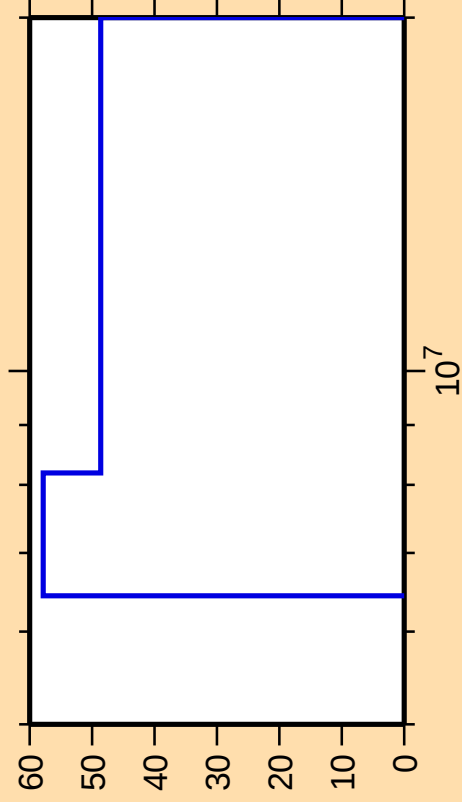
\Delta\sigma/\sigma vs. E for ^{158}\text{Tb}(n,p)
