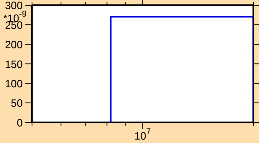
\sigma vs. E for ^{158}\text{Tb}(n,2np)
