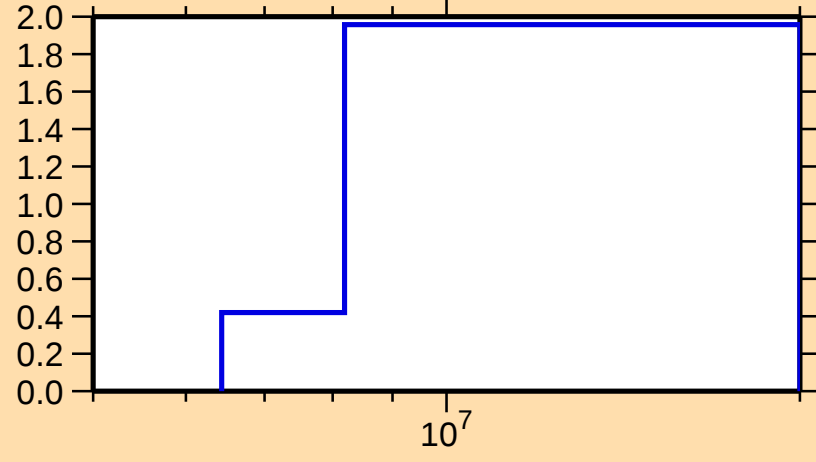
\sigma vs. E for ^{158}\text{Tb}(n,2n)
