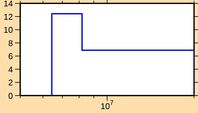
\Delta\sigma/\sigma vs. E for ^{158}\text{Tb}(n,2n)
