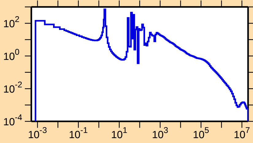
\sigma vs. E for ^{164}\text{Tb}(n,\gamma)
