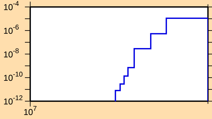
\sigma vs. E for ^{164}\text{Tb}(n,\text{nd})
