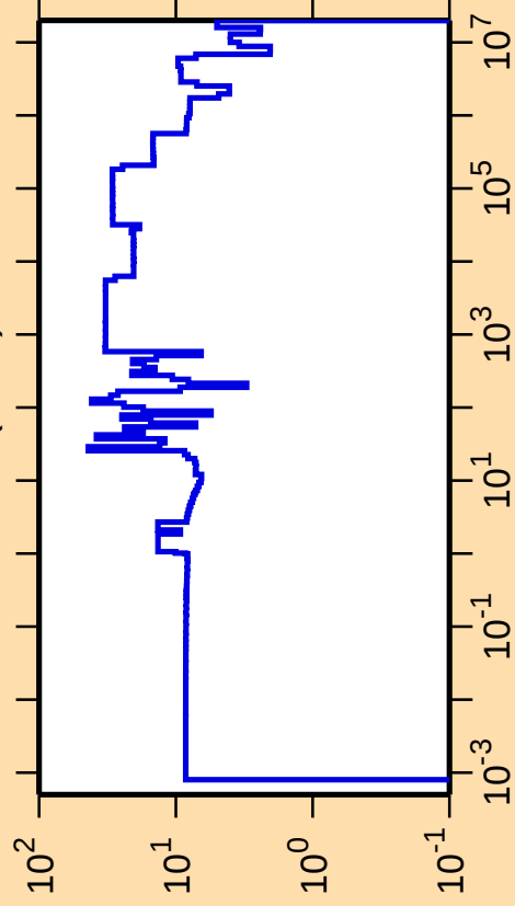
\Delta\sigma/\sigma vs. E for ^{164}\text{Tb}(n,\text{el.})
