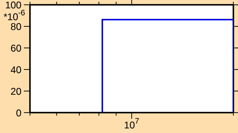
\sigma vs. E for ^{164}\text{Tb}(n,np)
