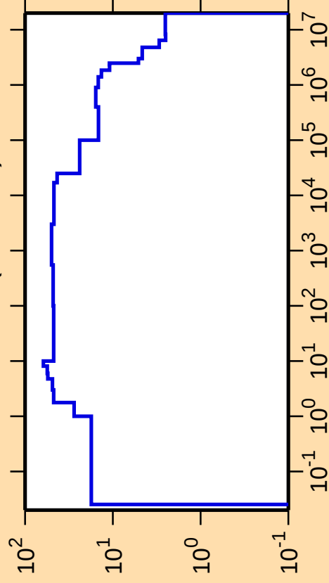
\Delta\sigma/\sigma vs. E for ^{164}\text{Tb}(n,\text{nonel.})
