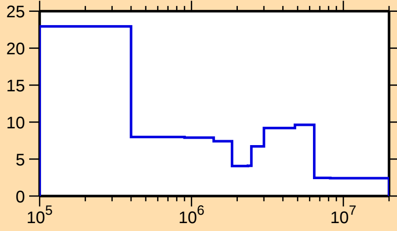
\Delta\sigma/\sigma vs. E for ^{164}\text{Tb}(n,\text{el.})
