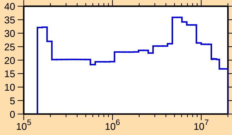
\Delta\sigma/\sigma vs. E for ^{167}\text{Tb}(n,\text{el.})
