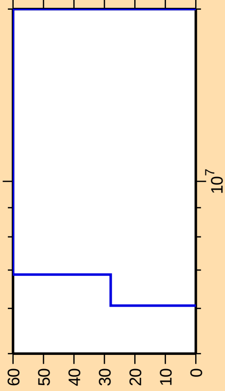
\Delta\sigma/\sigma vs. E for ^{167}\text{Tb}(n,n\text{cont.})
