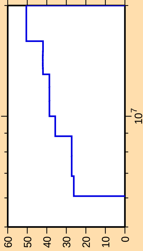
\Delta\sigma/\sigma vs. E for ^{167}\text{Tb}(n,n_1)
