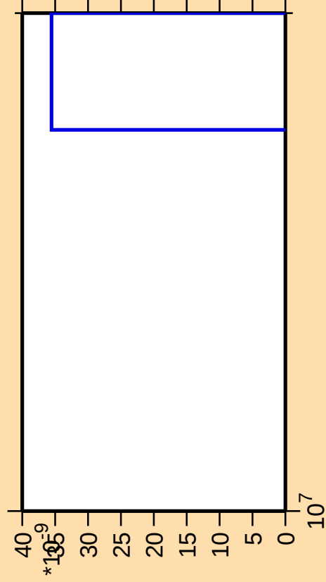
\Delta\sigma/\sigma vs. E for ^{167}\text{Tb}(\text{mt } 42)
