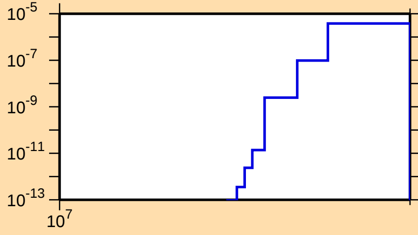
\sigma vs. E for ^{167}\text{Tb}(n,nt)
