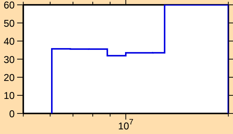
\Delta\sigma/\sigma vs. E for ^{167}\text{Tb}(n,2n)
