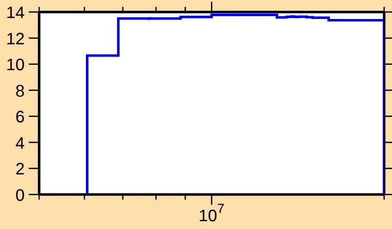
\Delta\sigma/\sigma vs. E for ^{167}\text{Tb}(n,\text{nonel.})
