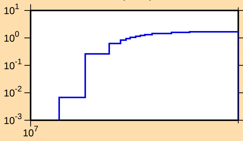
\sigma vs. E for ^{167}\text{Tb}(n,3n)
