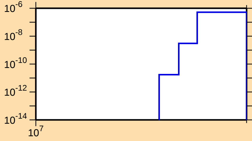
\sigma vs. E for ^{167}\text{Tb}(n,\text{nd})
