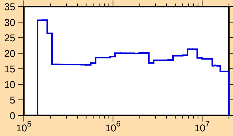
\Delta\sigma/\sigma vs. E for ^{167}\text{Tb}(n,\text{tot.})
