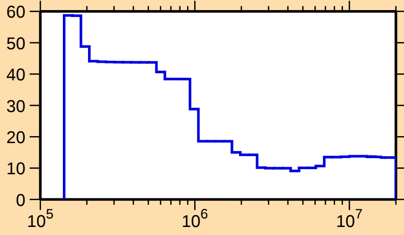
\Delta\sigma/\sigma vs. E for ^{167}\text{Tb}(n,n\text{onel.})
