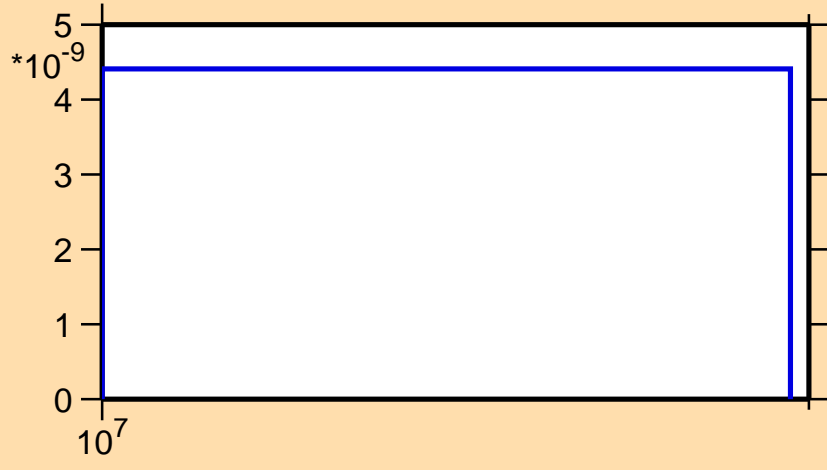
\sigma vs. E for ^{167}\text{Tb}(n,\text{nd})
