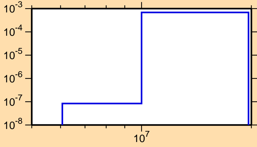
\sigma vs. E for ^{167}\text{Tb}(n,p)
