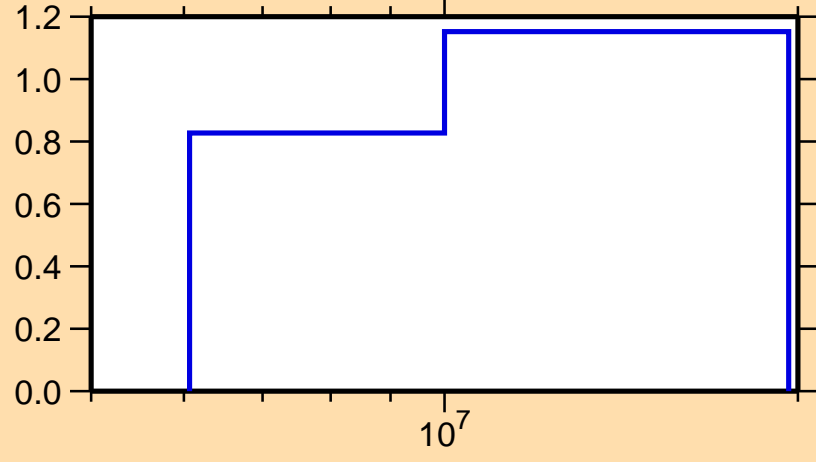
\sigma vs. E for ^{167}\text{Tb}(n,2n)
