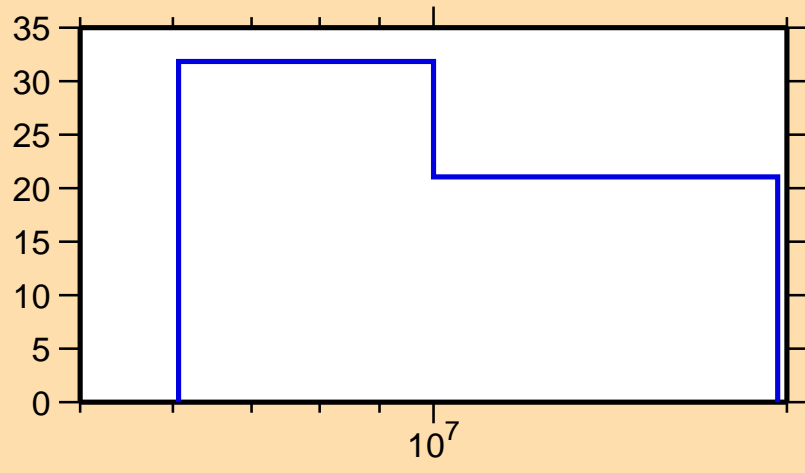
\Delta\sigma/\sigma vs. E for ^{167}\text{Tb}(n,el.)
