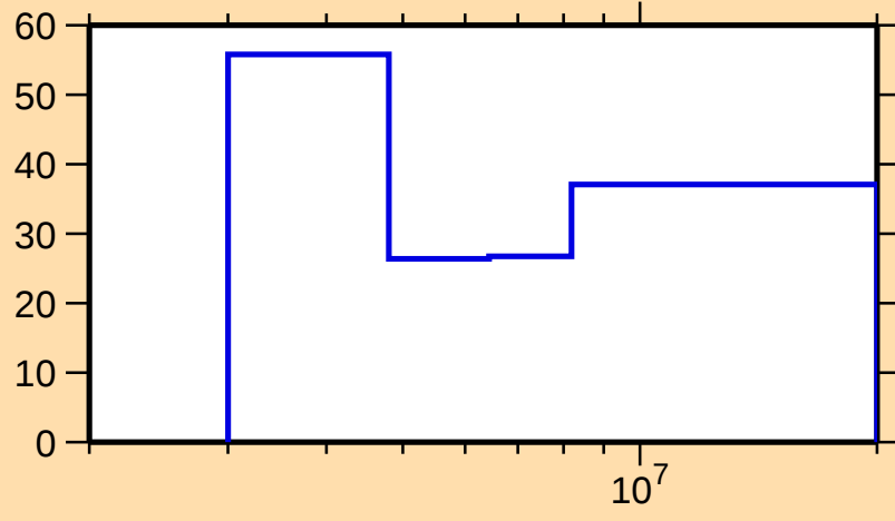
\Delta\sigma/\sigma vs. E for ^{167}\text{Tb}(n,n_1)
