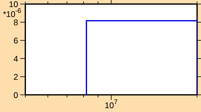
\sigma vs. E for ^{167}\text{Tb}(n,t)
