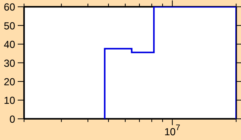
\Delta\sigma/\sigma vs. E for ^{167}\text{Tb}(n,2n)
