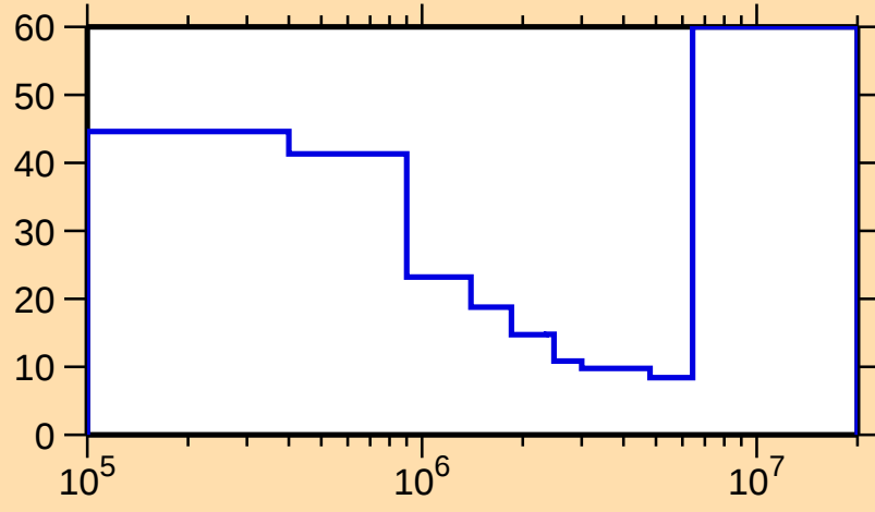
\Delta\sigma/\sigma vs. E for ^{167}\text{Tb}(n,\text{inel.})
