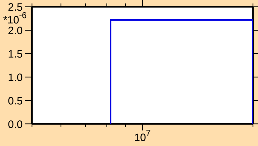
\sigma vs. E for ^{167}\text{Tb}(n,n\alpha)
