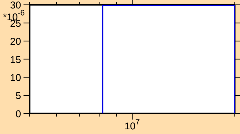
\sigma vs. E for ^{167}\text{Tb}(n,np)
