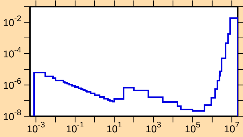
\sigma vs. E for ^{97}\text{Tc}(n,\alpha)
