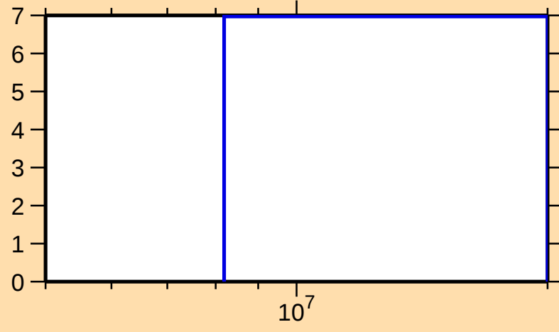
\Delta\sigma/\sigma vs. E for ^{97}\text{Tc}(n,\text{el.})
