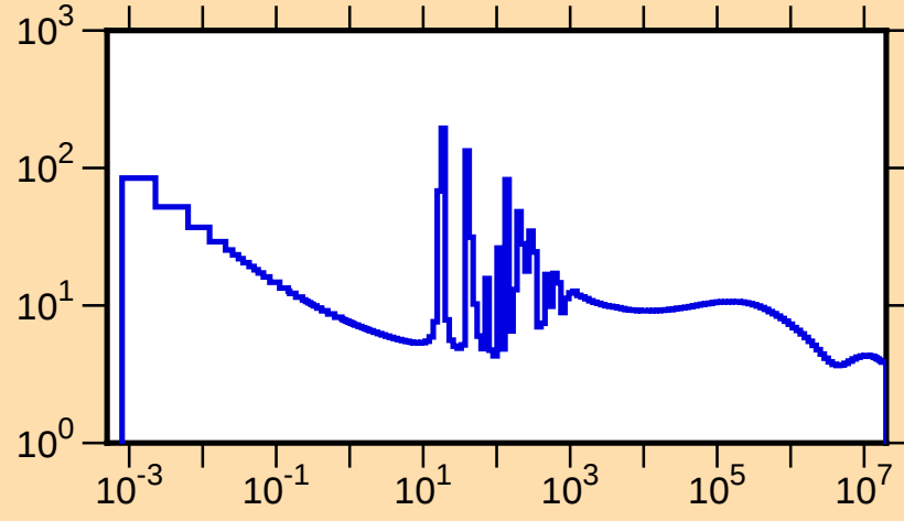
\sigma vs. E for ^{101}\text{Tc}(n,\text{tot.})
