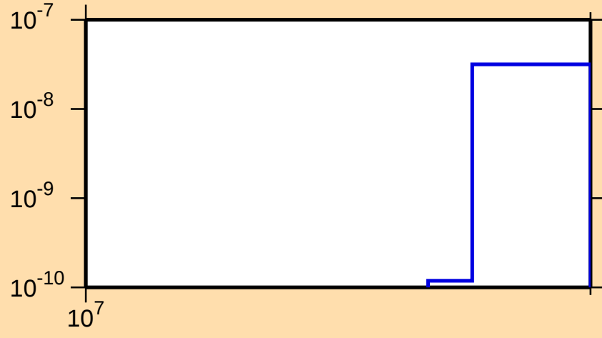
\sigma vs. E for ^{101}\text{Tc}(n,2n\alpha)
