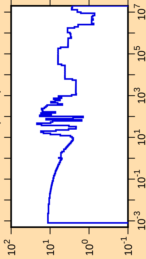
\Delta\sigma/\sigma vs. E for ^{101}\text{Tc}(n,\text{tot.})
