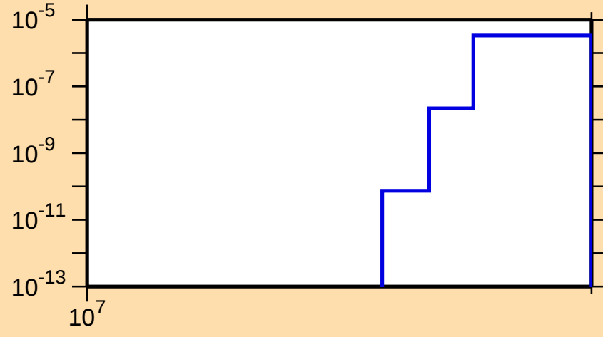
\sigma vs. E for ^{101}\text{Tc}(n,\text{nd})
